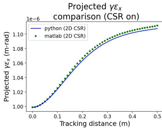
Figure 6: Projected horizontal beam emittance of a Gaussian bunch traversing a bend with 2D steady-state CSR wake applied from Python and Lucretia MATLAB.
