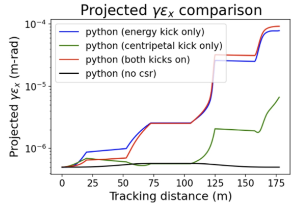
Figure 7: Projected horizontal beam emittance of a Gaussian bunch traversing the FACET-II chicane with 2D steady-state CSR wake applied from Python CSR2D.
