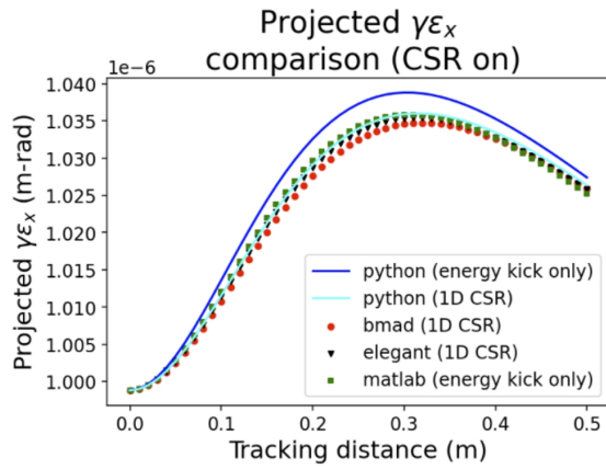
Figure 5: Projected horizontal beam emittance of a Gaussian bunch traversing a bend with steady-state CSR wake applied from different codes. With “energy kick only”, only the longitudinal kicks from the 2D CSR theory are applied.
