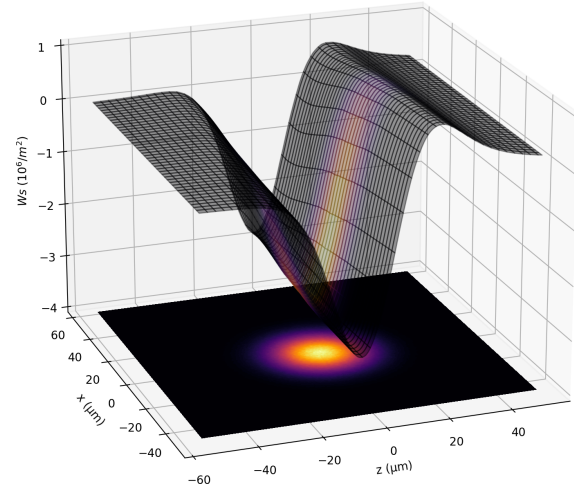
Figure 1: A typical contour plot of the longitudinal steady-state wake W_s(z, x) of a Gaussian bunch distribution.
