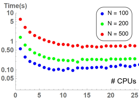
Figure 3: Timings to compute the \psi_s grid of size 2N -by- 2N .
