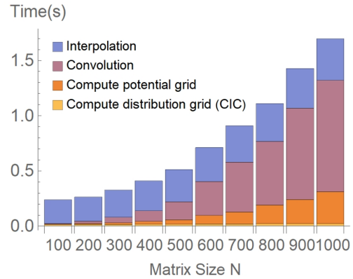
Figure 4: Timings for the four main steps to compute the W_s kicks on a million particles with a 2D grid size of N -by- N . Vectorization and Numba compiler are applied with 20 CPUs on Cori NERSC.
