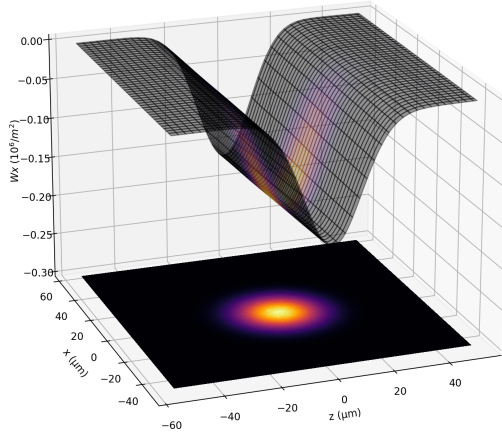
Figure 2: A typical contour plot of the horizontal steady-state wake W_x(z, x) of a Gaussian bunch distribution.
