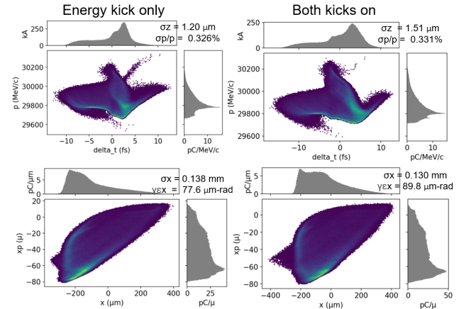
Figure 8: Longitudinal (top) and horizontal phase space (bottom) plots at the end of chicane tracking with either energy kick only (left) or both kicks on (right).
