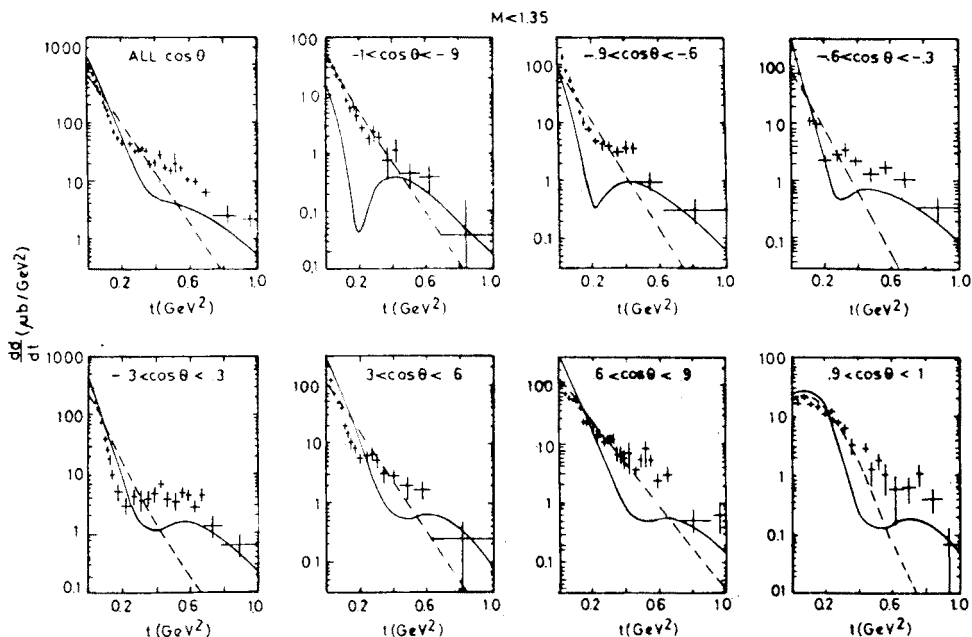
Fig. 4. Distributions in t_1 for M < 1.35 GeV. The solid theoretical curves are computed for M_{\text{TOT}} = M_\pi + M_{\text{abs}}^\pi and b_\pi = 2 \text{ GeV}^{-2} . Dashed lines show unabsorbed model ( M_{\text{TOT}} = M_\pi + M_N + M_D ) for b_\pi = 2 \text{ GeV}^{-2} , b_N = b_D = 1 \text{ GeV}^{-2} and are multiplied by 0.33 in order to make the integrated cross section agree with data
