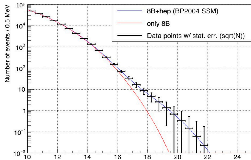
Figure 5. Expected HK recoil electron spectrum from solar neutrino-electron elastic scattering. Photocathode coverage is assumed to be 40%. The dominant {}^8\text{B} component (red) has a smaller endpoint than hep (the blue line shows {}^8\text{B} + hep combined).
