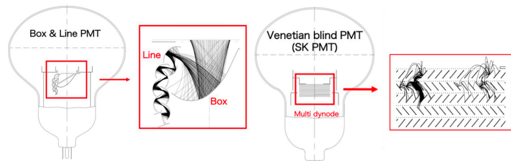
Figure 1. “Box and line” (left) and “Venetian blinds” (right) PMT [3].
