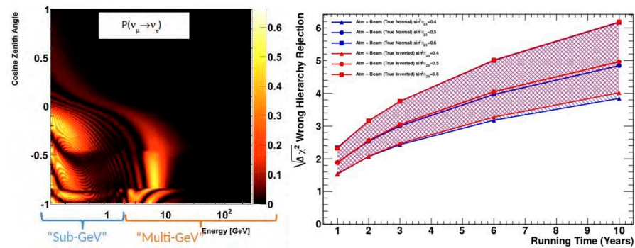
Figure 3. (Left): Atmospheric neutrino muon to electron flavor oscillation probability as a function of zenith angle and energy (normal ordering). (Right): Expected significance of the wrong mass ordering rejection as a function of HK running time.
