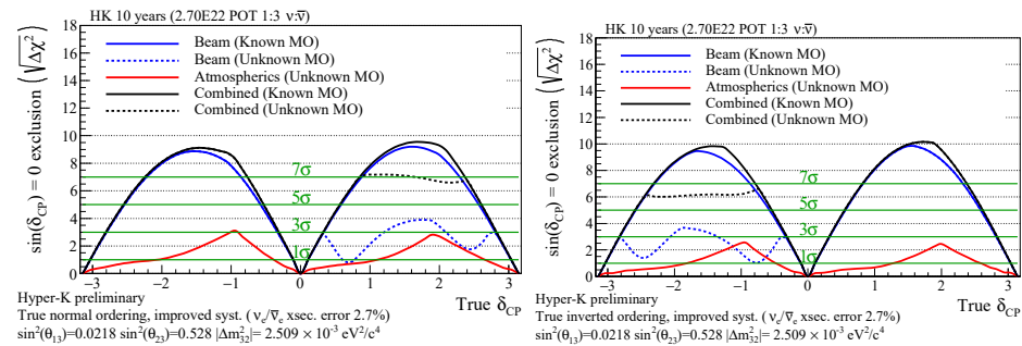
Figure 2. CP violation for known and unknown, normal and inverted mass ordering from beam neutrinos and the combination of beam and atmospheric neutrinos.
