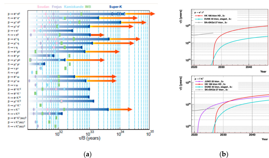
Figure 4. HK nucleon decay sensitivity: (a) Expected 90% C.L. limits for many modes in HK compared to Frejus, Kamiokande, IMB, SK, and HK. (b) Expected 90% C.L. limits for p \rightarrow e^+ \pi^0 and p \rightarrow K^+ \nu in HK compared to SK, JUNO, and DUNE.
