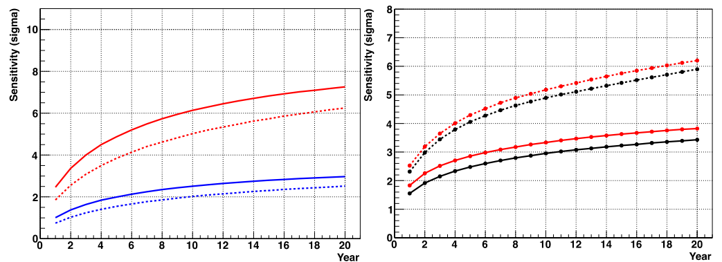
Figure 7. Left: Sensitivity of HK to find a non-zero day/night asymmetry (red) and separate predictions based on the solar and KamLAND best-fit \Delta m^2_{21} values. Solid lines are for 40% photocathode coverage and dotted lines for 20%. Right: Sensitivity of HK to find significant spectral distortions due to the MSW effect. The solid (dashed) lines are for a 3.5 MeV (4.5 MeV) threshold of recoil electron kinetic energy. The black (red) line assumes the best solar neutrino \Delta m^2_{21} fit of 2019 (2020).
