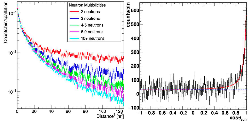
Figure 6. Left: Distance 3 of the “center of gravity” of “neutron clouds” from hadronic showers with the observed radioactive decays. Right: Angular distribution of additional solar neutrino recoil electron candidates with respect to the solar direction after employing new tagging methods.
