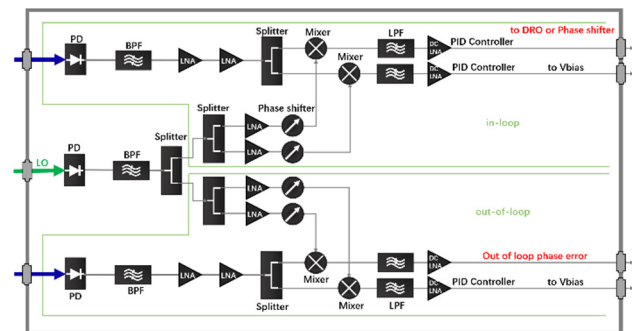
Figure 2: The simplified block diagram of the electronics.
