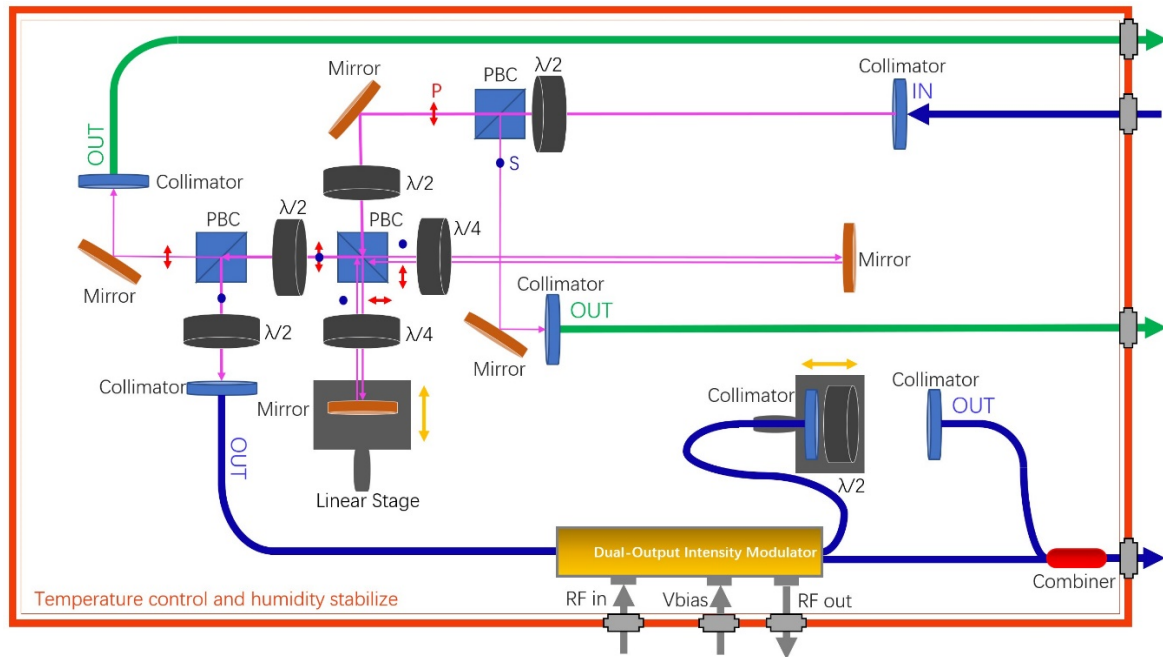
Figure 1: Diagram of the optical part.
