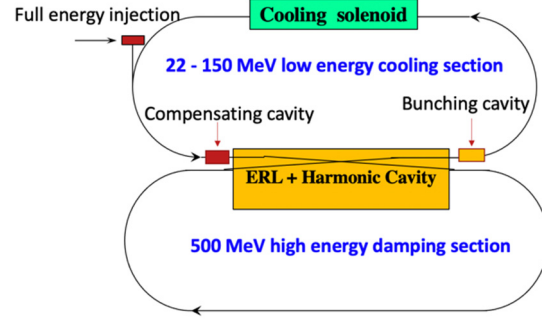
Figure 1: Schematic drawing of a dual-energy storage ring cooler.
