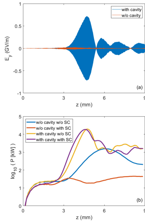
Figure 2: (a) temporal signature of the radiated field value sampled on-axis in front of the bunch for trapped and free electrons, and (b) radiated power on logarithmic scale versus undulator length for free and trapped electrons with and without considering space-charge effect.
