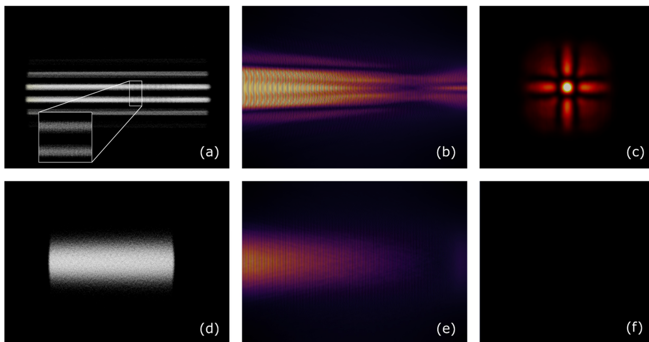
Figure 3: Visualization of the simulation results at the instant of maximum radiated power: (a) bunch profile, (b) field profile, and (c) beam power profile in front of the bunch for confined electrons, and (d) bunch profile, (e) field profile, and (f) beam power profile in front of the bunch for free electrons.
