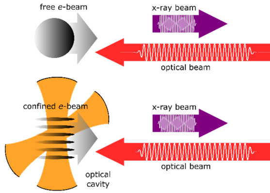
Figure 1: Schematic illustration of optical undulator with confined electrons compared to free electrons.
