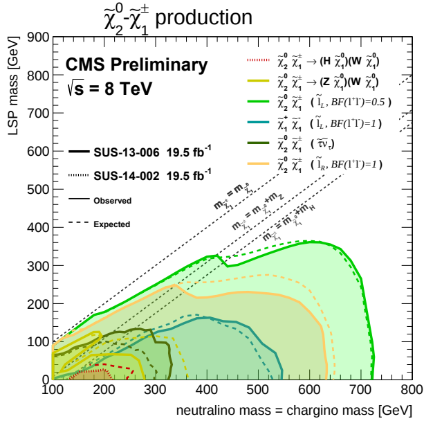
Fig. 2. Summary of CMS searches for electroweak production of charginos and neutralinos based on 19.5/fb of pp collision data at \sqrt{s} = 8 TeV [1, 5].
