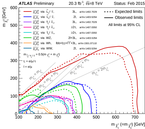
Fig. 3. Summary of ATLAS searches for electroweak production of charginos and neutralinos based on 20/fb of pp collision data at \sqrt{s} = 8 TeV [6, 7].
