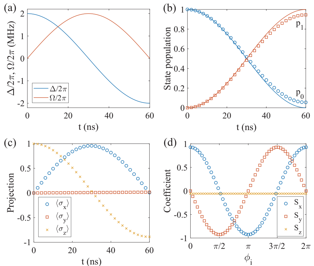
Figure 2. (a) The scheme for implementing the quantum state transfer by time-dependent parameters of the driving pulse. (b) The state populations of spin qubit 2 during the quantum state transfer process, with spin qubit 1 and 2 initially in |1\rangle and |0\rangle . The solid line is the evolution without environmental noises and the dotted line is the evolution with environmental noises. (c) The quantum state tomography of spin qubit 2 involves projecting the state onto the Pauli matrices \sigma_x, \sigma_y and \sigma_z . (d) The coefficients S_x, S_y and S_z of the states of spin qubit 2 as a function of initial phase \phi_i in the quantum state transfer, with spin qubit 1 initially in (|0\rangle + e^{i\phi_i}|1\rangle)/\sqrt{2} .
