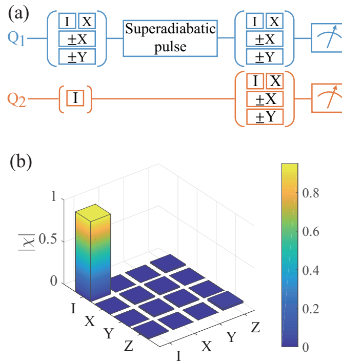
Figure 3. (a) The whole pulse sequence is used to characterize the quantum state transfer between the two spin qubits. We prepare six mutually unbiased states of spin qubit 1, while spin qubit 2 is in state |0\rangle . Next, we apply a superadiabatic pulse to transfer the state of spin qubit 1 to spin qubit 2. Finally, we obtain the quantum state tomography of the system through joint readout. (b) The process matrix of the state transfer in the basis \{I, X, Y, Z\} using the quantum process tomography, and the fidelity reaches F = 95.1\% .
