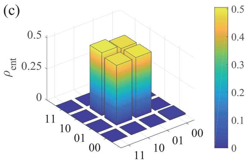
Figure 5. (a) The whole pulse sequence is used to generate remote entangled states between spin qubits using our scheme. The spin qubits 1 and 2 can initially be in states |1\rangle and |0\rangle , and then we perform a well-designed superadiabatic pulse. Finally, we obtain the density matrix of the system through quantum state tomography. (b) The average value of the Pauli operators \langle \sigma_i \sigma_j \rangle for the spin qubits. (c) The density matrix \rho_{ent} of the generated remote entangled state and the state fidelity is F_{ent} = 97.6\% relative to the ideal Bell state.
