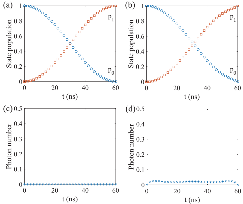
Figure A1. The state population of spin qubit 2 during the quantum state transfer process is obtained using (a) the effective Hamiltonian and (b) the full Hamiltonian. (c,d) correspond to the remaining excited photon number in the resonator, respectively. Here, we neglect the influence of the environmental noises.
