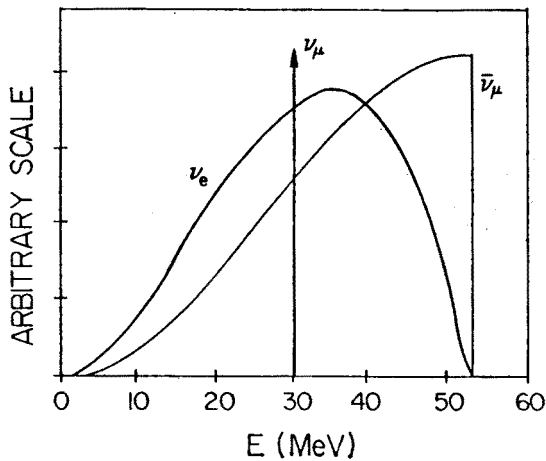
Fig. 6. Neutrino spectra from beam stop \pi^+ \rightarrow \mu^+ + \nu_\mu \downarrow \rightarrow e^+ + \nu_e + \bar{\nu}_\mu
