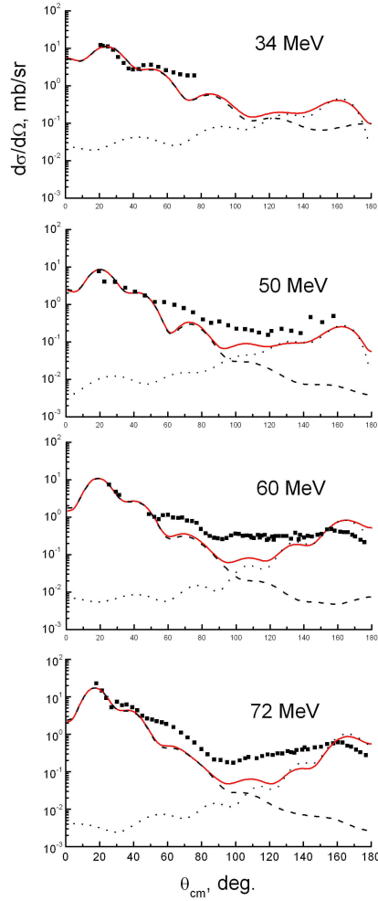
Fig. 4. The angular distributions of the ^3\text{He} ions scattered on ^6\text{Li} nuclei at 34, 50, 60 and 72 MeV energies with excitation of the 2.186 MeV ( 3^+ ) state. All notations are the same as in Fig. 3.
