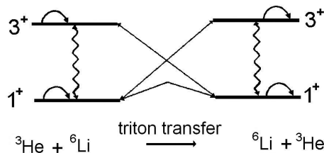
Fig. 1. The coupling scheme used in the coupled reaction channels calculations of {}^3\text{He} scattering by {}^6\text{Li} nuclei.
