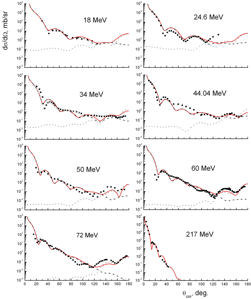
Fig. 3. The angular distributions of ^3\text{He} ions elastically scattered on ^6\text{Li} nuclei at 34, 50, 60 and 72 MeV energies. Open circles are experimental data obtained in the present work, square points are data taken from [11–15, 17, 24]. Curves are the results of calculations by the coupled reaction channels method. Solid curves are calculations with taking into account all couplings at the coherent addition of scattering and triton transfer mechanisms. Dashed curves are calculations with the coupling of the elastic and inelastic scattering only. Dotted curves are calculations for the triton exchange mechanism.
