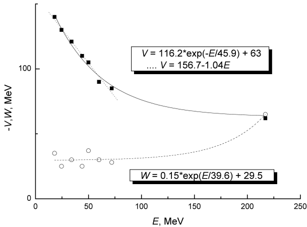
Fig. 2. The energy dependence of the real (■) and imaginary (○) depths of potentials found.
