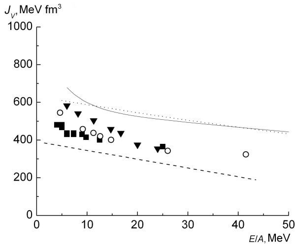
Fig. 5. The energy per nucleon ( E/A ) dependence of the volume integrals of the real potentials ( J_V ), found from the analysis of the scattering for {}^3\text{He} + {}^6\text{Li} (this work ( \blacktriangledown )), d + {}^6\text{Li} [19] ( \blacksquare ) and \alpha + {}^6\text{Li} [18] ( \circ ) systems. Curves are approximations of the energy dependence of J_V for p + {}^6\text{Li} [26] (dotted), {}^3\text{He} + {}^6\text{Li} [4] (solid), and {}^{12}\text{C} + {}^{12}\text{C} [27] (dashed) systems.
