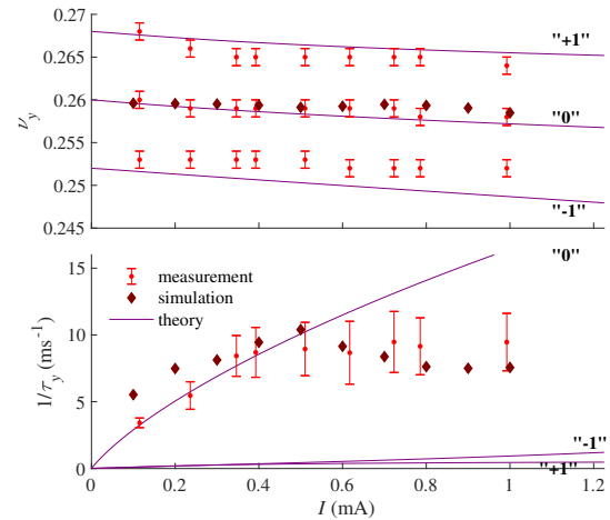
Figure 5: Frequencies (top) and damping/growth rates (bottom) of vertical head-tail modes; \xi_y = 2.1 ; feedback on.
