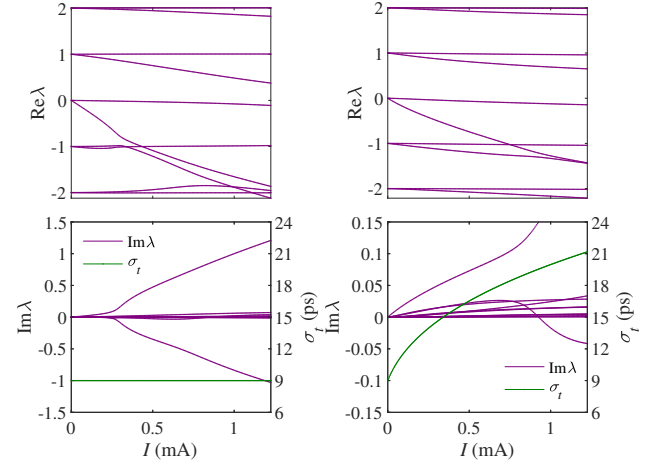
Figure 2: Effect of bunch lengthening on the frequencies (top) and damping/growth rates (bottom) of the 10 lowest vertical modes.
