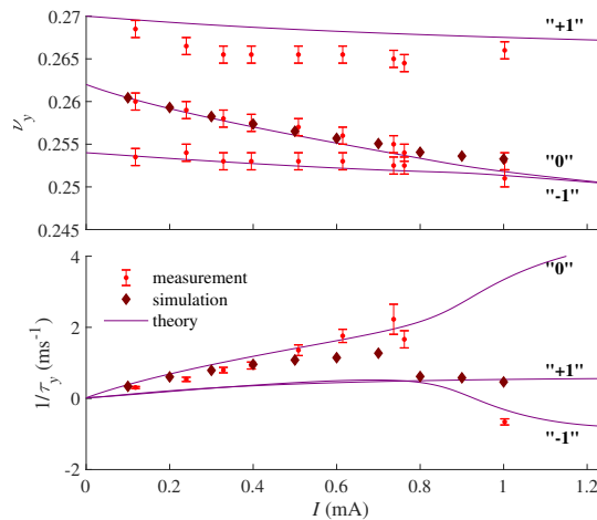
Figure 4: Frequencies (top) and damping/growth rates (bottom) of vertical head-tail modes; \xi_y = 2.1 ; feedback off.
