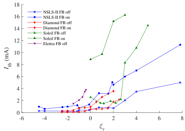
Figure 1: Measured single-bunch threshold current as a function of chromaticity, with and without feedback.
