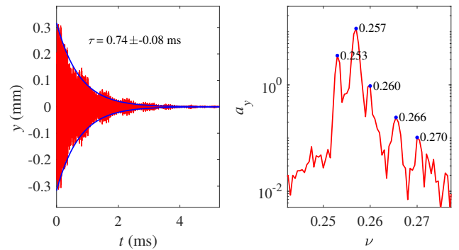
Figure 3: Vertical turn-by-turn oscillation (left) and its spectrum (right); \xi_y = 2.1 ; I_b = 0.5 mA.
