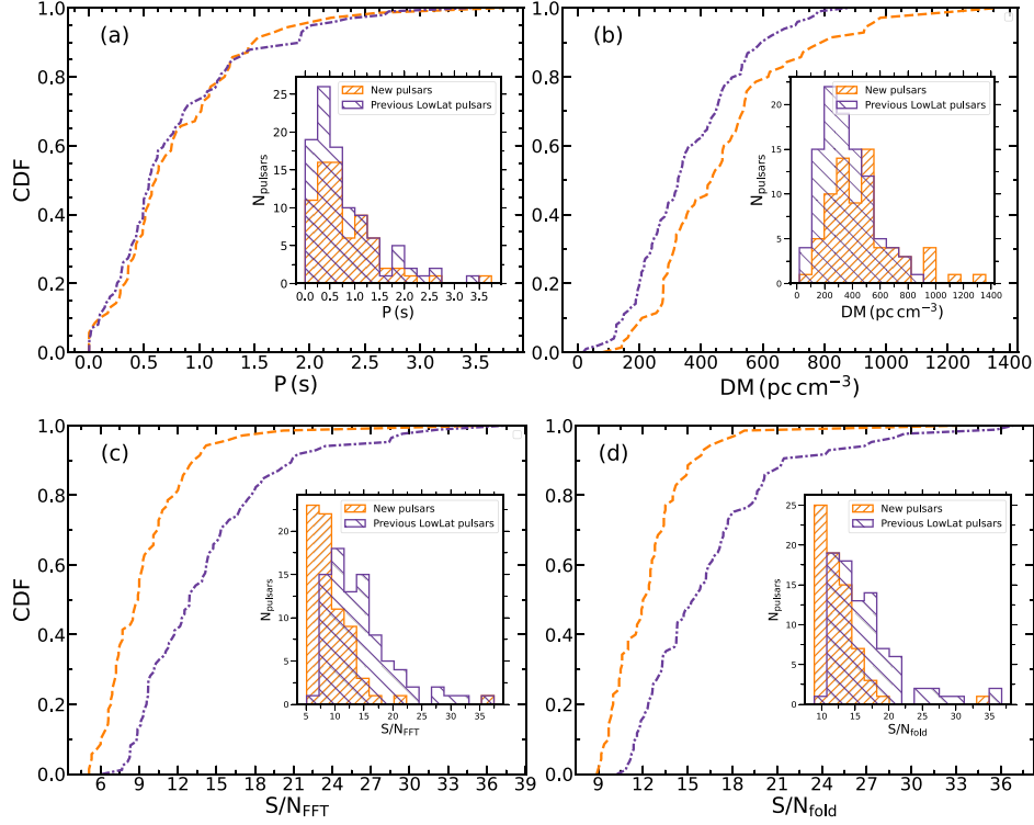
Figure 3. Spin period, DM, S/N_{\text{FFT}} , and S/N_{\text{fold}} distributions of previously discovered HTRU-S LowLat pulsars (violet) and the new pulsar sample (red) reported in this paper. Each plot shows the cumulative distribution function of each distribution, and inside each plot are histograms of the corresponding distribution.
