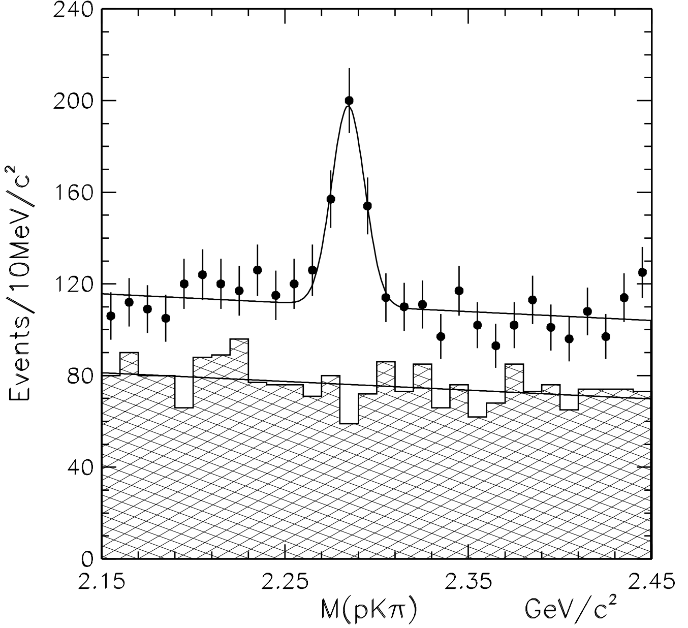
FIG. 1. Invariant mass of pK^-\pi^+ for right sign (points with error bars) and wrong sign events (shaded area). The fit yields of 197 \pm 25 right sign events. There is no evidence of a \Lambda_c signal in wrong sign combinations. The signal region is defined to be 2.260 – 2.308 \text{GeV}/c^2 and the two sideband regions are 2.176 – 2.224 \text{GeV}/c^2 and 2.376 – 2.424 \text{GeV}/c^2 .
