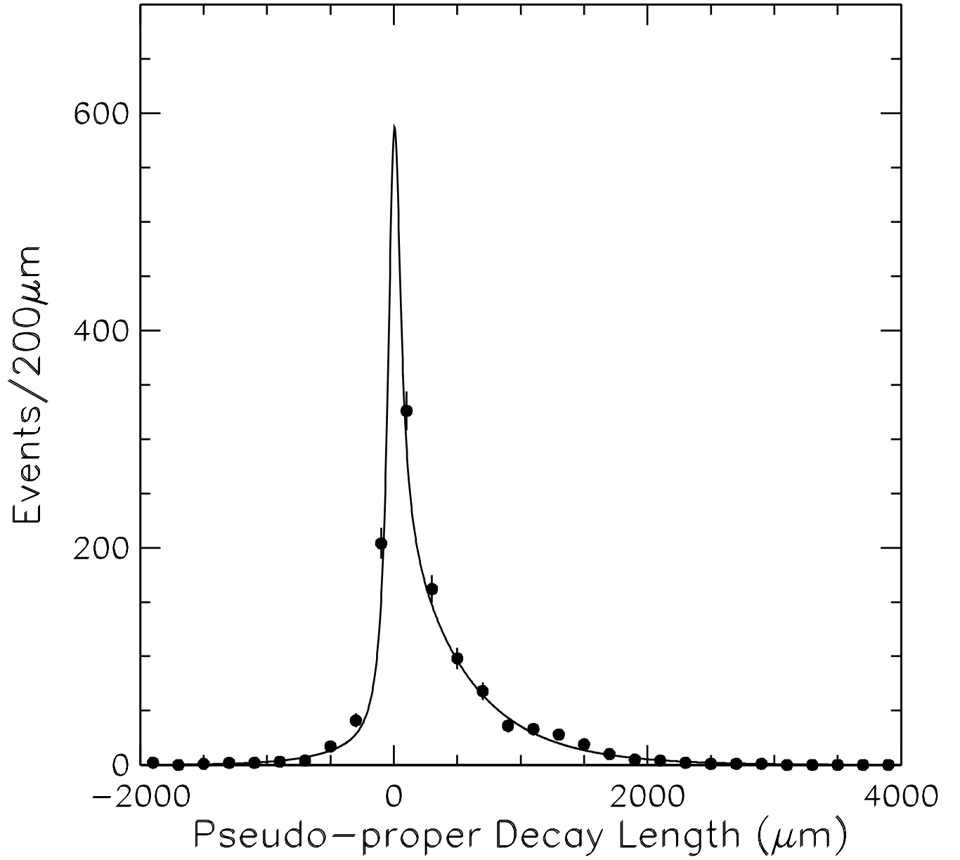
FIG. 3. Pseudo-proper decay length distribution from the pK^-\pi^+ invariant mass sideband sample. The points with error bars are data points and the solid line is the fit result. Most of this background is from b-hadron decays.
