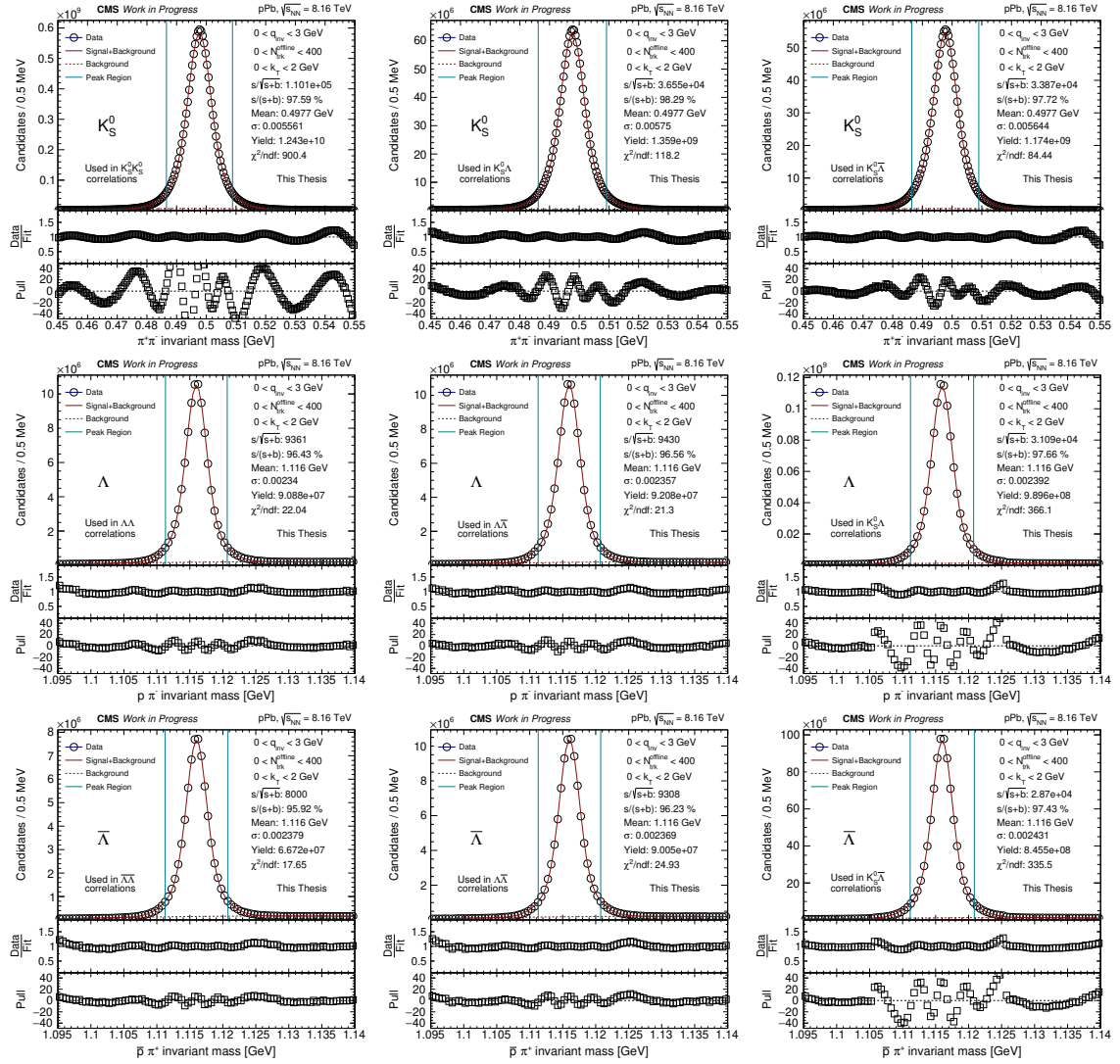
Figure 5.12: Examples of invariant mass distributions (including fits) integrated in q_{inv} ( 0 < q_{inv} < 3 \text{ GeV} ), k_T ( 0 < k_T < 2 \text{ GeV} ) and multiplicity ( 0 < N_{trk}^{offline} < 400 ), for K_S^0 (top panel), \Lambda 's (middle panel) and \bar{\Lambda} 's (bottom panel) used in different correlations. More informations in the text.
