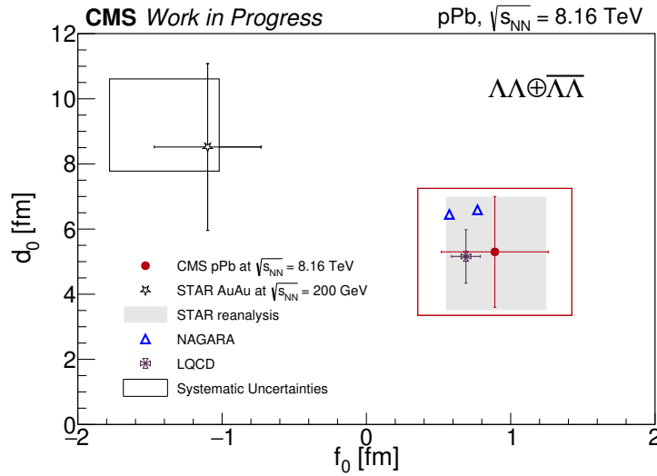
Figure 6.6: Scattering observables, d_0 versus f_0 , extracted using Lednický-Lyubolshitz model for \Lambda\Lambda \oplus \bar{\Lambda}\bar{\Lambda} pairs in pPb collisions at \sqrt{s_{\text{NN}}} = 8.16 \text{ TeV} (red marker), compared with Lattice QCD results [210, 332] (purple marker) and previous measurements from STAR at AuAu collisions at \sqrt{s_{\text{NN}}} = 200 \text{ GeV} [240] (black marker), STAR reanalysis [241] (gray area) and NAGARA events [238, 239] (blue markers).
