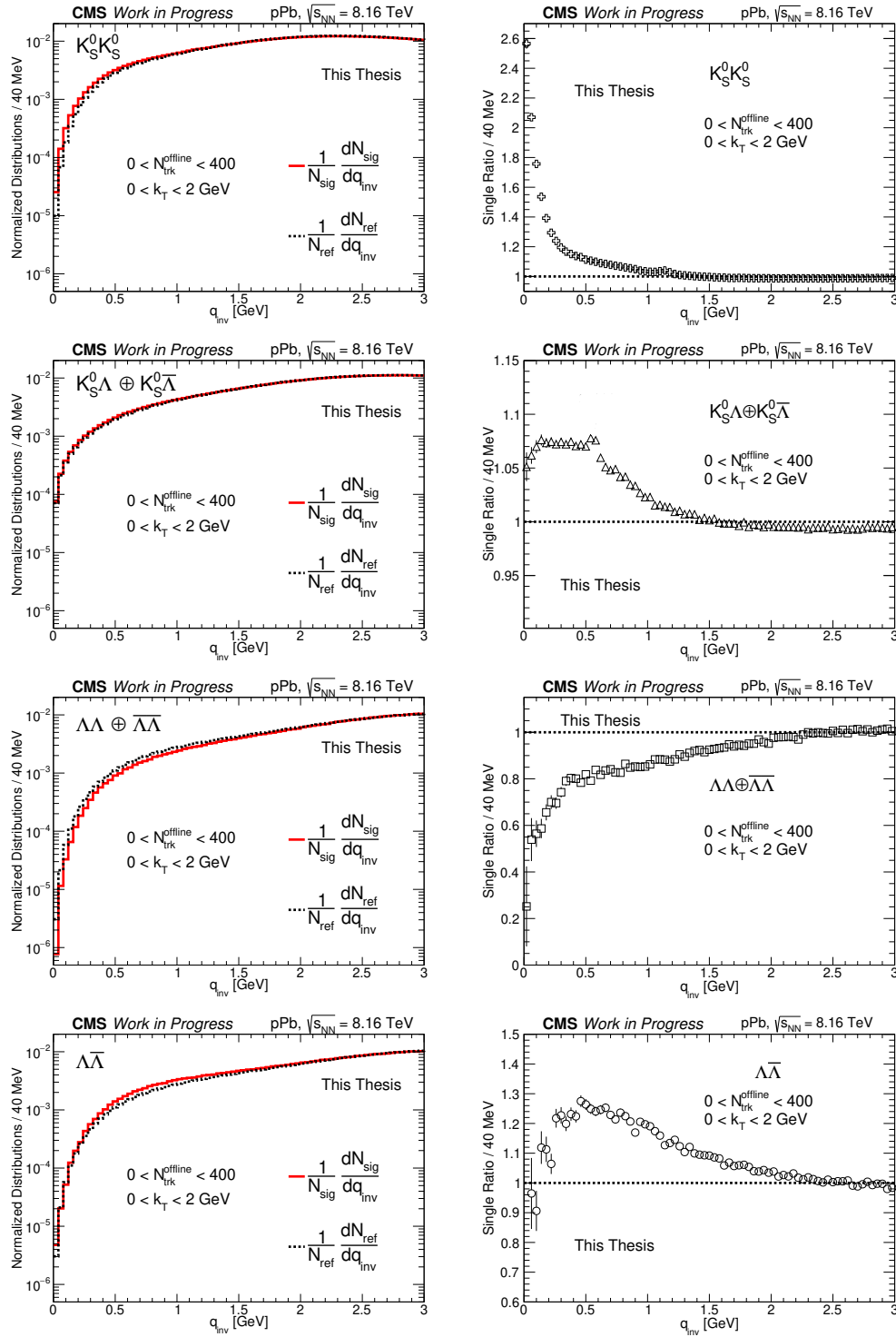
Figure 5.16: Normalized distributions for signal and reference sample (left panel) and single ratio (right panel) as function of q_{\text{inv}} integrated in k_T ( 0 < k_T < 2 GeV) and multiplicity ( 0 < N_{\text{trk}}^{\text{offline}} < 400 ), for K_S^0 K_S^0 (top panel), K_S^0 \Lambda \oplus K_S^0 \bar{\Lambda} (middle-top panel), \Lambda \Lambda \oplus \bar{\Lambda} \bar{\Lambda} (middle-bottom panel) and \Lambda \bar{\Lambda} (bottom panel). The SR plots are shown in different scales in the y-axis to emphasize the different effects.
