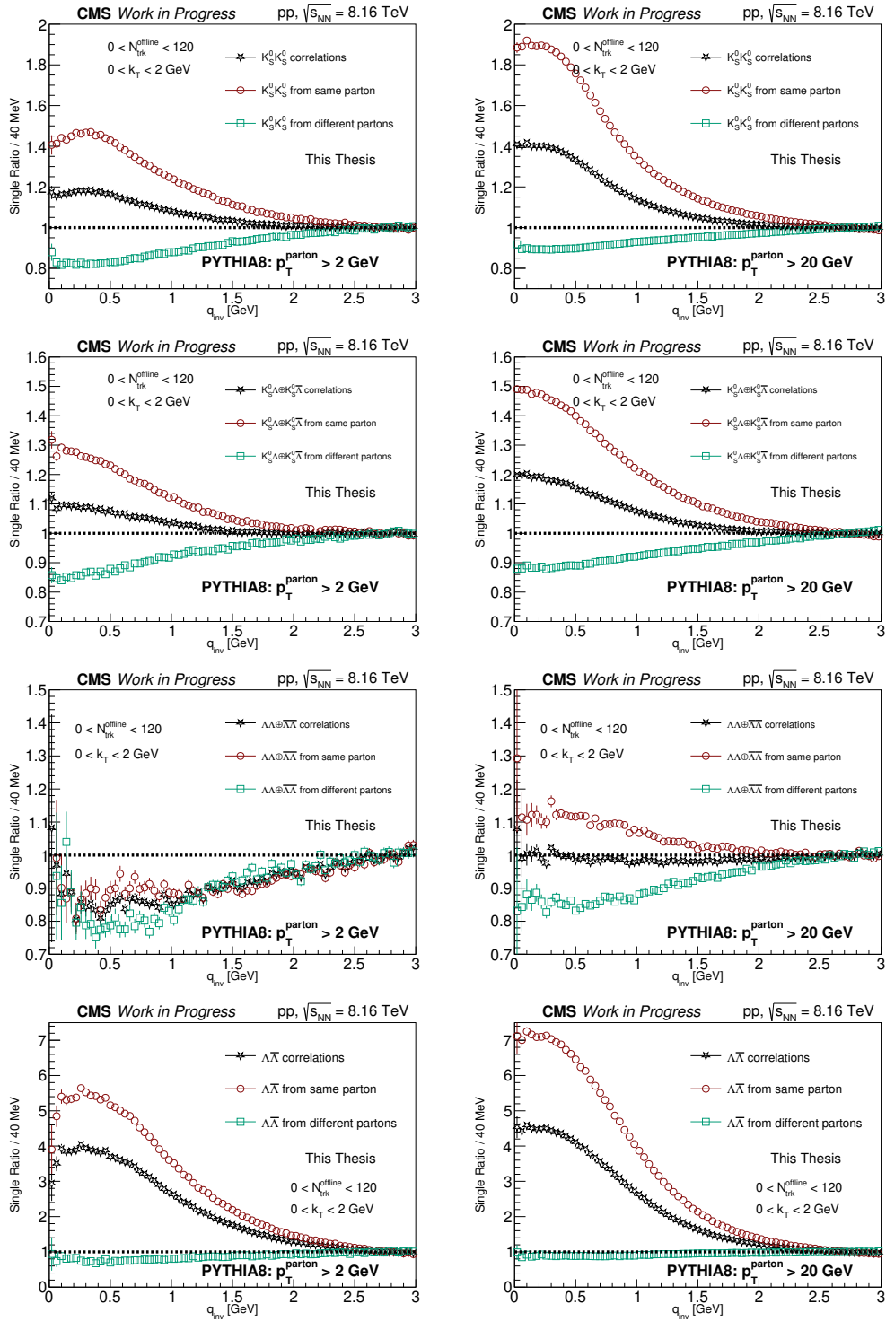
Figure 5.21: Single ratios as function of q_{inv} calculated using PYTHIA8 , in two different regimes: p_T^{\text{parton}} > 2 \text{ GeV} (left panel) and p_T^{\text{parton}} > 20 \text{ GeV} (right panel); for K_S^0 K_S^0 (top panel), K_S^0 \Lambda \oplus K_S^0 \bar{\Lambda} (middle-top panel), \Lambda \Lambda \oplus \bar{\Lambda} \bar{\Lambda} (middle-bottom panel) and \Lambda \bar{\Lambda} (bottom panel). The usual correlations (black open star) are compared with the cases where V^0 comes from same (open green circles) and different (open green squares) partons.
