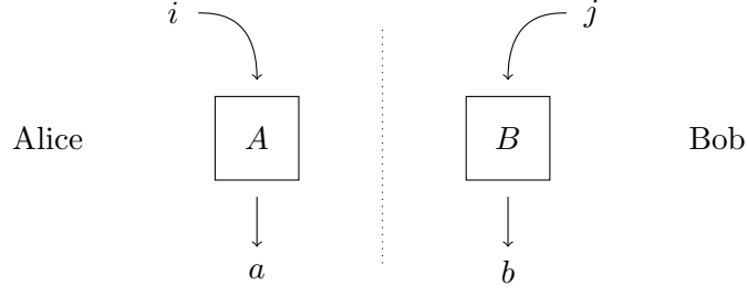
Figure 1: A pictorial representation of PR boxes. The boxes A and B represent a physical system made of two space-like separated subsystems, the random variables i and j label the possible choices of experiments and the variables a and b the possible outcomes. The vertical line reminds of the fact that we are assuming A and B to be space-like separated.
