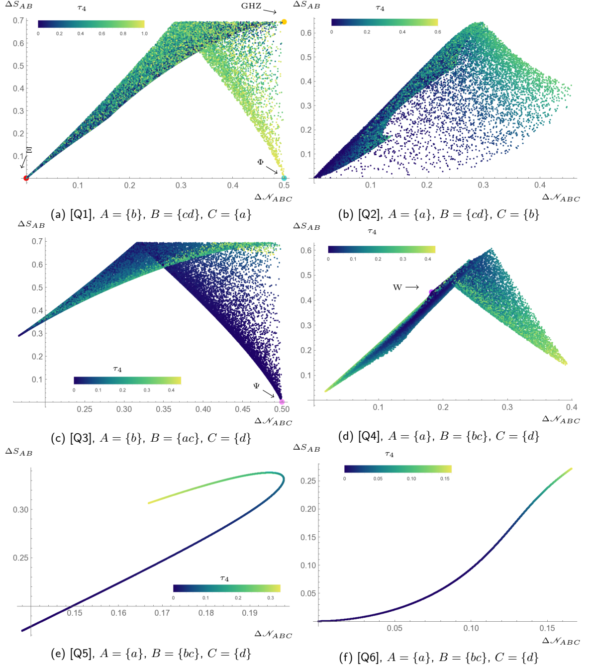
Figure 8: Disentangling theorem and saturation of Araki-Lieb (see Eq. (4.4.26)) for the SLOCC classified 4-qubit states (50000 random states per class). The large dots show the GHZ (orange), |\Phi\rangle (turquoise), |\Psi\rangle (pink), W (purple) and maximally entangled |\Xi\rangle (red) states.
