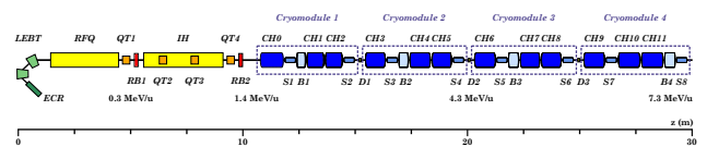
Figure 6: Layout of the HELIAC accelerator.
