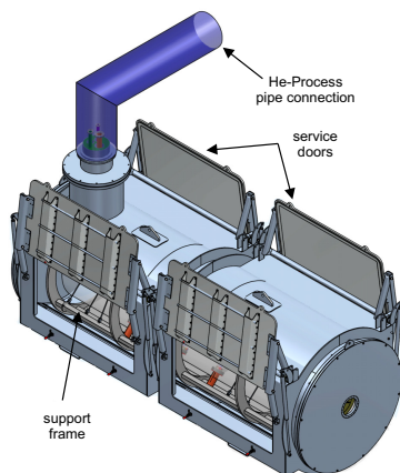
Figure 5: 3-D model of the Advanced Demonstrator cryomodule.
