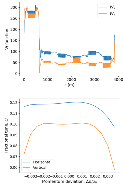
Figure 2: W -functions along the ring and tune as a function of momentum offset using two global sextupole families to correct the linear chromaticity.
