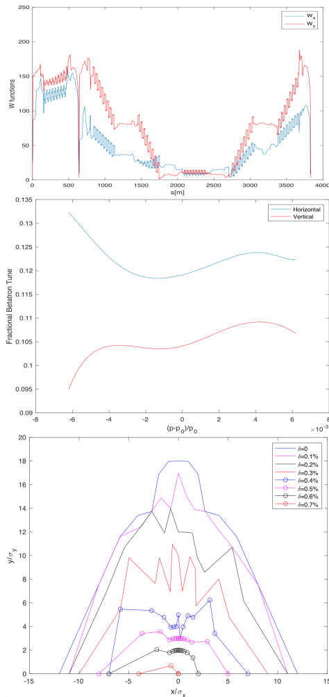
Figure 3: W -functions along the ring (top), tune as a function of momentum offset (middle), and dynamic aperture (bottom) using fourteen sextupole families over the ring. The dynamic aperture is computed in LEGO [11] with RF on and without synchrotron radiation.
