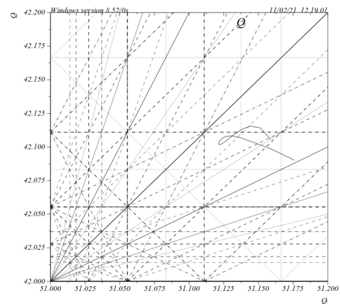
Figure 4: Resonance diagram ( Q_x, Q_y ) with an example of a tune footprint superimposed.
