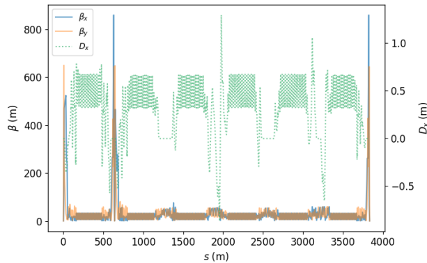
Figure 1: Linear optics functions for the ESR 2-IP lattice. The ring consists of six arcs, separated by straight sections. The beams collide at IP6 ( s = 0 ) and IP8 ( s = 641 m).
