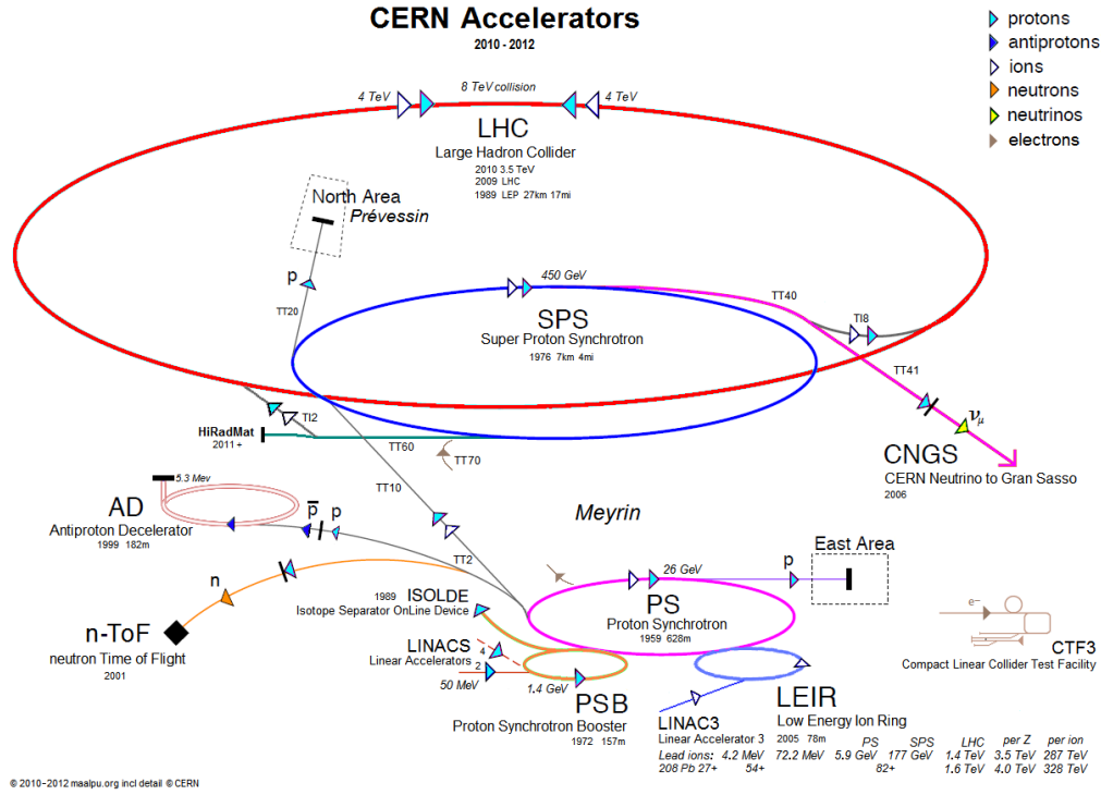
Figure 2.1: A schematic diagram of the LHC accelerator complex.
