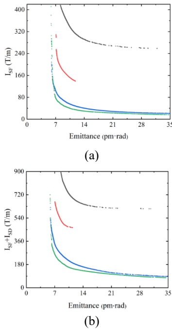
Figure 2: Pareto front of the integrated strength of sextupoles and beam emittance. (Black: standard unit cell; Red: Complex unit cell with two main bends; Blue: Complex unit cell with three main bends; Green: Complex unit cell with four main bends).
