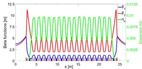
Figure 5: Linear optical functions of the 17BA lattice based on the standard unit cell.
