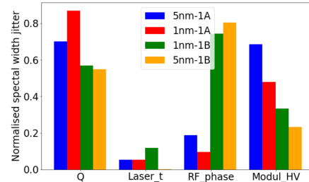
Figure 4: Comparison of normalised spectral width jitter from beam parameters.
