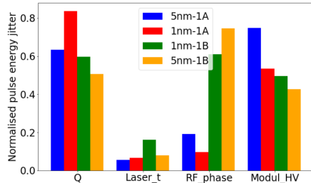
Figure 2: Comparison of normalised pulse energy from beam parameters.
