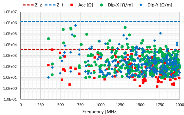
Figure 3: HOM impedances of the 197 MHz RFD cavity.
