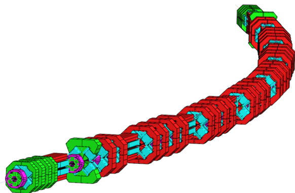
Figure 4: Layout of the magnets for one full sector of the ring.
