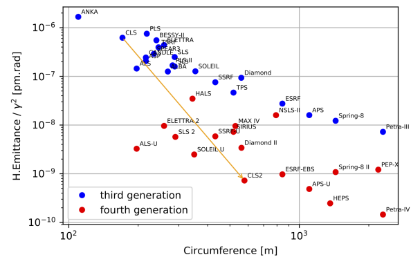
Figure 3: CLS2 design circumference and normalised horizontal emittance compared with other existing third and fourth generation light sources in operation and planned upgrades. The arrow shows the dramatic improvement in performance of the ring design from CLS to CLS2 (adapted from Ref. [6]).
