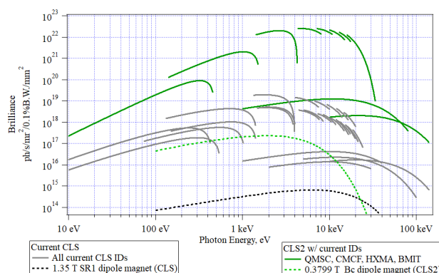
Figure 2: Brilliance curve comparison of CLS and CLS2 with the existing CLS ID designs.
