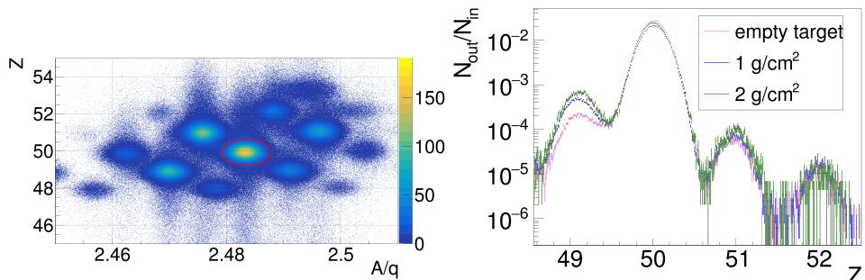
Fig. 2. (Colour on-line) Left: Incoming particle identification by Z and A/q measurements. ^{124}\text{Sn} is indicated by a red/grey ellipse. Right: Comparison of outgoing particle counts in R3B-MUSIC ( N_{\text{out}} ), normalized to the number of incoming particles ( N_{\text{in}} ), for measurements with and without the target.
