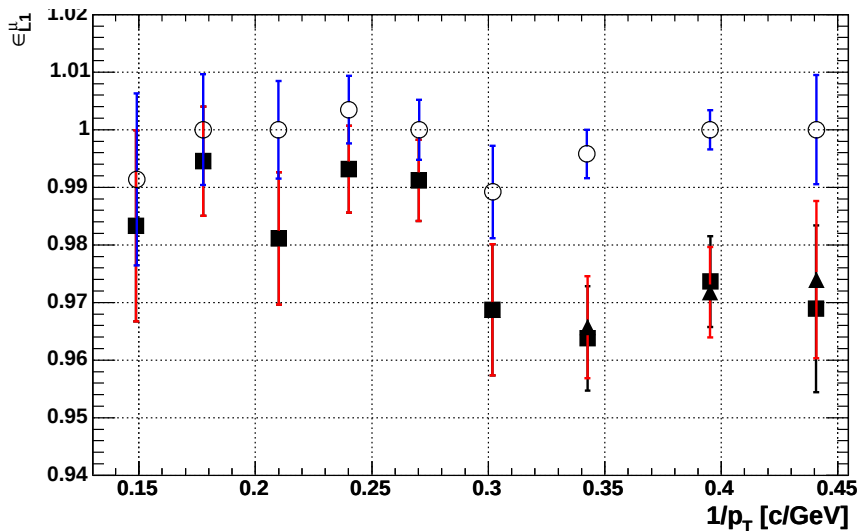
FIG. 73: L1 CMX source of inefficiency for XFT 2-miss period: \epsilon_{\text{stub,CMX}}^\mu (▲), \epsilon_{\text{XTRP,CMX}}^\mu (○), and \epsilon_{\text{CMX}}^\mu (■).
