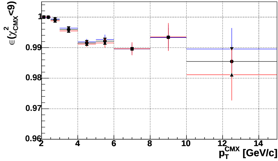
FIG. 52: \epsilon(\chi^2_{r\phi,CMX} < 9) vs. p_T : \mu^+ ( \blacktriangle ), \mu^- ( \blacktriangledown ), and charge averaged ( \bullet ).
