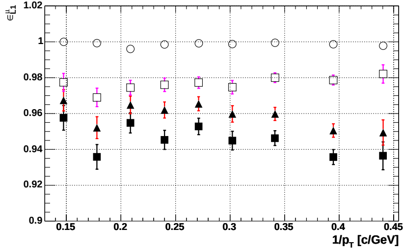
FIG. 79: L1 CMX source of inefficiency for XFT 1-miss period (ranges #3-#5 combined only): \epsilon_{\text{stub,CMX}}^\mu (▲), \epsilon_{\text{XTRP,CMX}}^\mu (○), \epsilon_{\text{CSX,CMX}}^\mu (□), and \epsilon_{\text{CMX}}^\mu (■).
