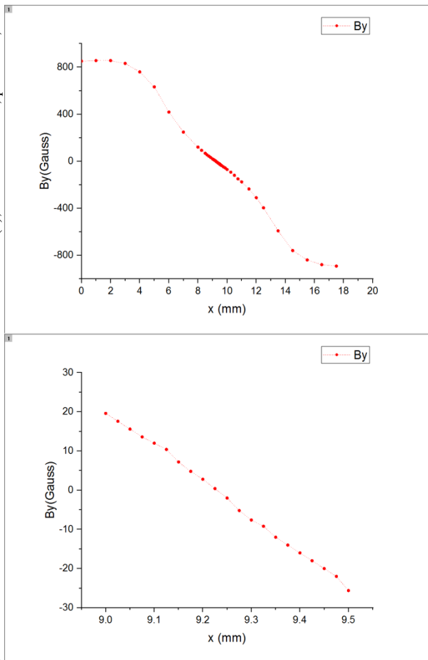
Figure 5: The magnetic field along horizontal direction and a horizontal zoom of magnetic field in central region.
