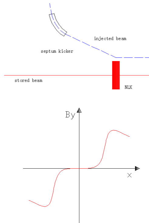
Figure 1: The layout of single pulse nonlinear kicker injection (the injected beam is deflected by the septum magnet into the NLK) and a diagram of magnetic field distribution in NLK.
