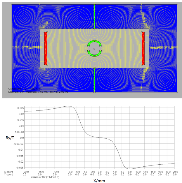
Figure 3: Simulation by OPERA2D and the magnetic field line Distribution in the NLK.
