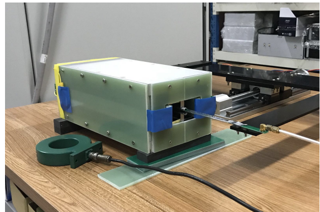
Figure 4: Measurement of the prototype.
