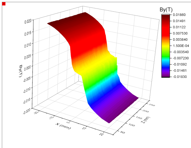
Figure 2: Simulation by OPERA3D and the magnetic field in the By direction on the XZ plane.
