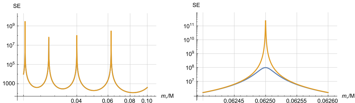
Figure 1. SE vs m_*/M for the Hulthén potential. Left: naive SE given by S(v) of eq. (3.6), corresponding to the usual computation in the literature. The regulated SE computed from eq. (2.39) is superimposed, but the difference from the usual method is invisible on the scale of the plot. Right: zoom-in on one of the resonant SE peaks. The regulated SE obtained from eq. (2.39) is the smooth lower curve below the sharp peak of the naive S(v) . For this plot, we took \alpha = 1 , v = 10^{-6} , and short-range annihilation and elastic cross sections \sigma v_0 = 1/(32\pi M^2) and \sigma_{sc,0} = (\mu^2 \sigma v_0 / 4\pi) \sigma v_0 .
