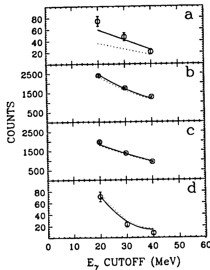
FIG. 4. Number of radiated events versus the cutoff energy \omega' , in the intervals -60^\circ < \theta_\gamma < -20^\circ [radiation along the proton direction (a)], -20^\circ < \theta_\gamma < 20^\circ [radiation along the incident electron direction (b)], 20^\circ < \theta_\gamma < 50^\circ [radiation along the scattered electron direction (c)], and the region 50^\circ < \theta_\gamma < 90^\circ (d). The solid (dotted) curve shows the prediction in the soft-photon limit for Bethe-Heitler and VC contributions (Bethe-Heitler only).
