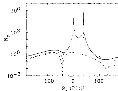
FIG. 3. Angular distribution of radiated photons in the single-photon limit. No acceptance effects are taken into account. The various curves denote the \delta_{ee} (dotted), \delta_{ep} (dot-dashed), and \delta_{pp} (dashed) contributions. The solid curve shows the coherent sum of the various contributions.
