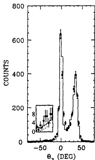
FIG. 2. Calculated angular distribution of radiated events in comparison with NE-18 data for \omega' > 30 MeV. The solid (dotted; see inset) curve shows the prediction in the soft-photon limit for Bethe-Heitler and VC contributions (Bethe-Heitler only). The central angle \theta_\gamma for the incident (scattered) electron and outgoing proton are 0^\circ ( 37.29^\circ ) and -43.29^\circ , respectively. Note that the inset shows the region -60^\circ < \theta_\gamma < -20^\circ with a different vertical scale.
