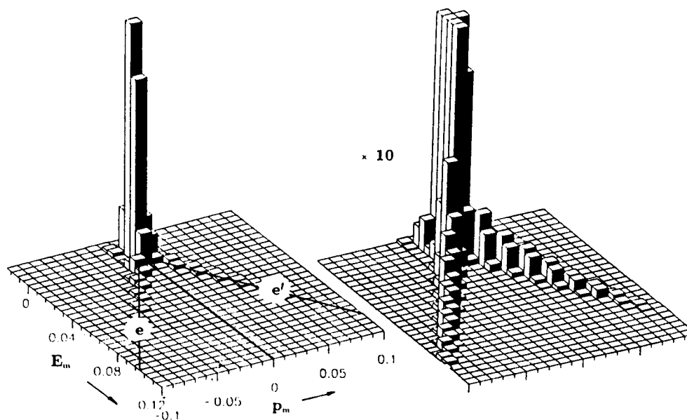
FIG. 1. Event distribution versus E_m and p_m (in GeV) without radiative corrections for the reaction ^1H(e, e'p) . The two radiative tails due to photon emission of the electron before and after the interaction can be observed. The sign of p_m is + (−) in case the angle of p_m , with respect to the incident electron, is < (>) \theta_e/2 .
