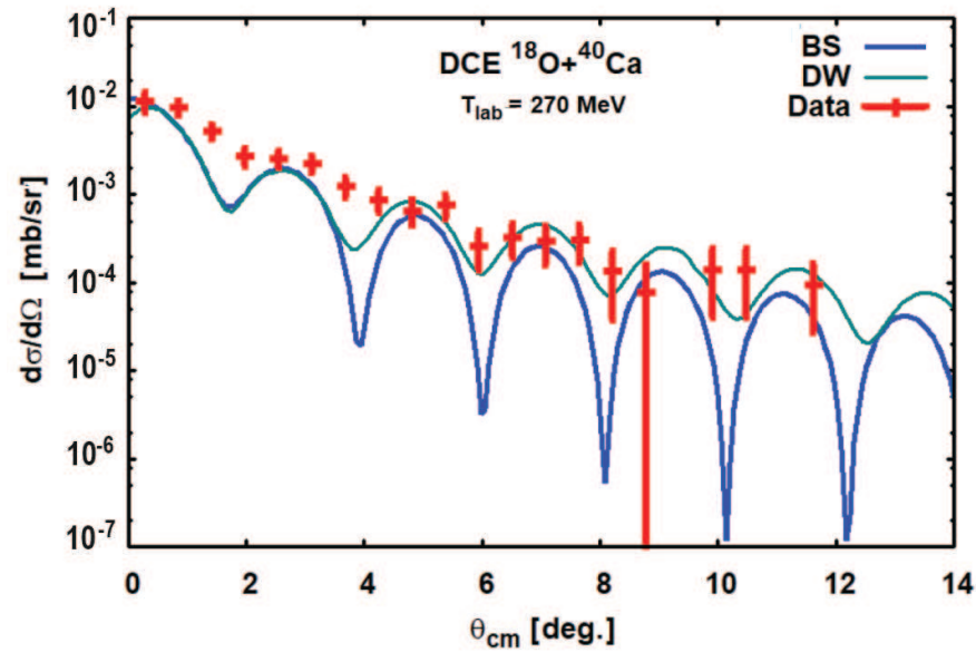
Figure 4. Second-order black sphere (BS, bold blue line) results for the reaction ^{40}\text{Ca}(^{18}\text{O}, ^{18}\text{Ne})^{40}\text{Ar} at T_{\text{lab}} = 270 MeV are compared to data from [32] and the full second-order DW results from Ref. [29] (DW, grey thin line). The BS results are normalized to the DW results by a \chi^2 fit.
