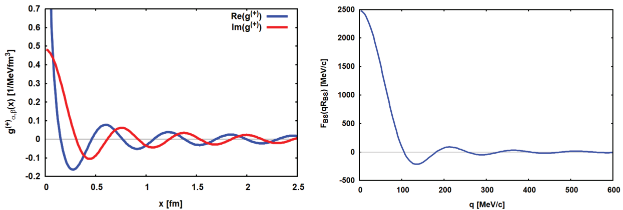
Figure 3. The propagator g_{\alpha\beta}^{(+)}(x) for the reaction ^{40}\text{Ca}(^{18}\text{O}, ^{18}\text{Ne})^{40}\text{Ar} at T_{lab} = 270 MeV with k_0 \sim 2017 MeV/c is shown on the left. The real part (blue) and the imaginary part (red) are shown separately. On the right, the black sphere distribution for the BS radius R_{abs} = 8.40 fm is displayed.
