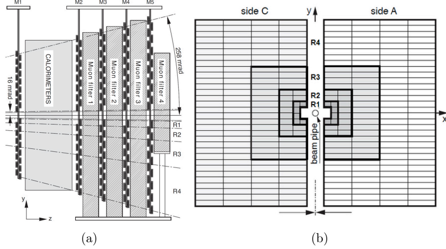
Figure 2.12: Schematic side view of the muon system (a) and structure of a single station (b).
