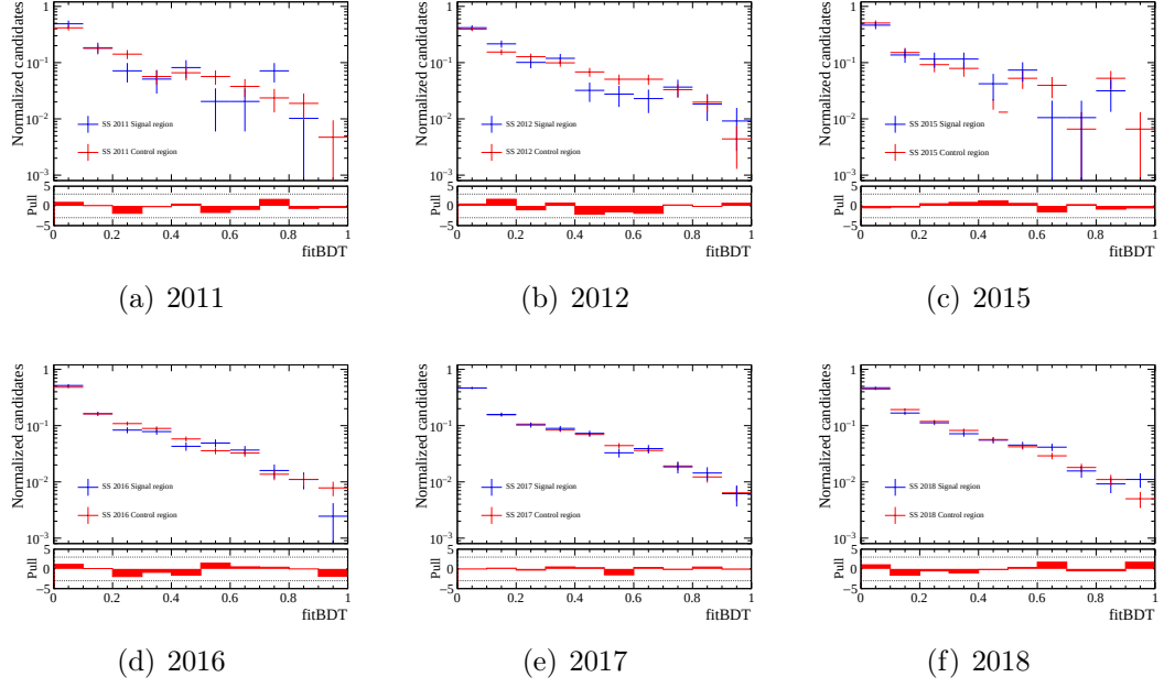
Figure 10.1: Comparison of the 3\pi 3\pi fitBDT distribution in signal and control regions for SS data in logarithmic scale.
