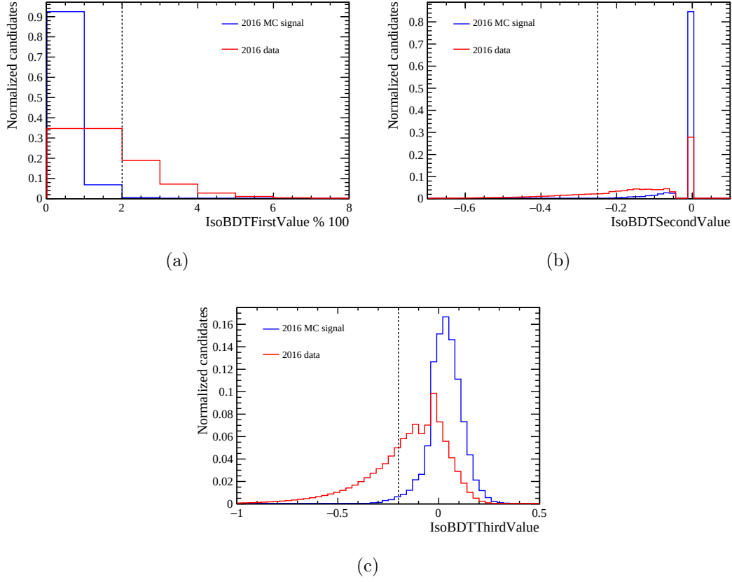
Figure 5.10: Distribution of IsoBDTFirstValue % 100 (a), IsoBDTSecondValue (b) and IsoBDTThirdValue (c) for the pion from the K^{*0} for the 3\pi 3\pi final state in 2016 data (red) and fully-matched MC (blue).
