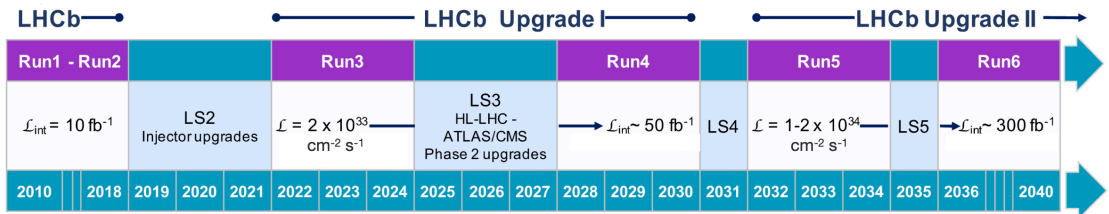
Figure 2.16: Timeline for the LHC.
