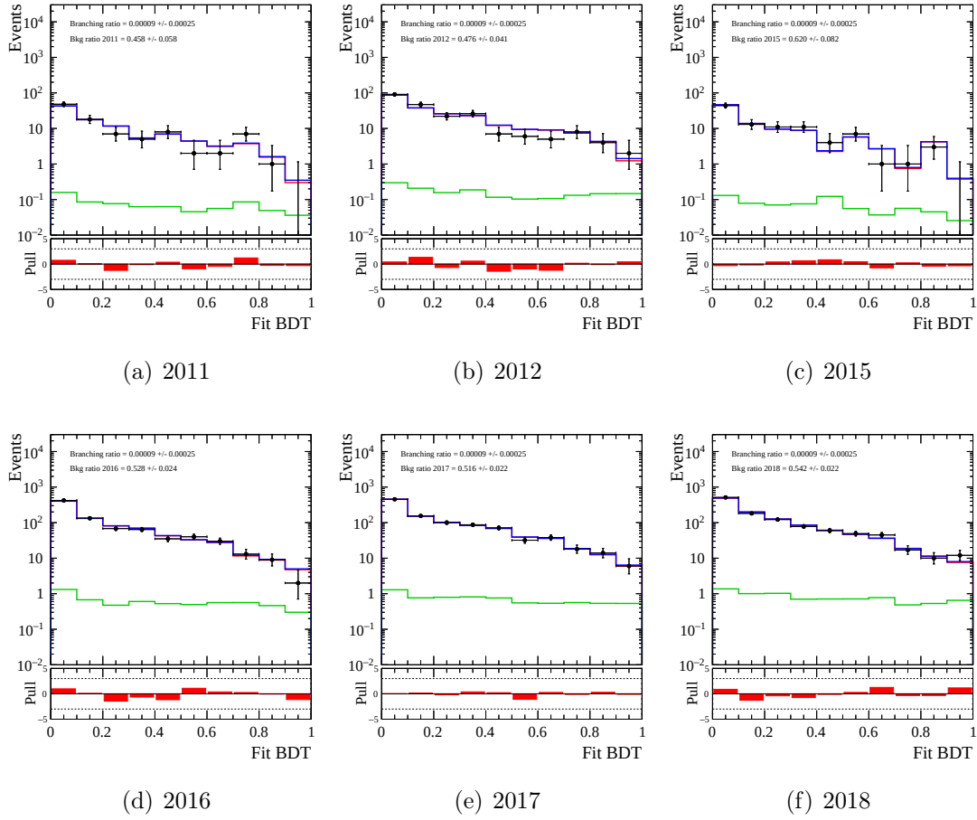
Figure 10.2: Result of the simultaneous fit over the data-taking years of 3\pi 3\pi SS data. Shown are the data (black points), the signal (green), the background (red) and the total PDF (blue).
