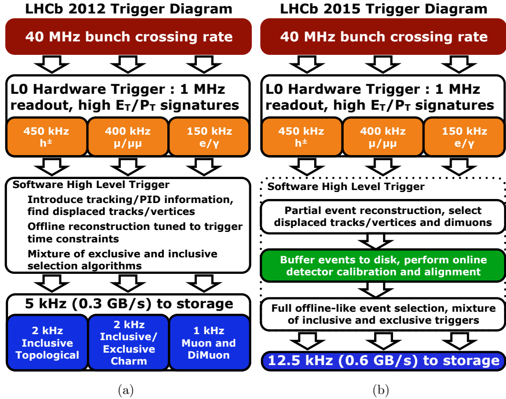
Figure 2.15: Trigger workflow in Run 1 (a) and Run 2 (b).
