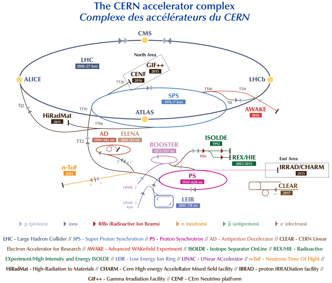
Figure 2.2: Schematic view of the CERN accelerator complex [78].
