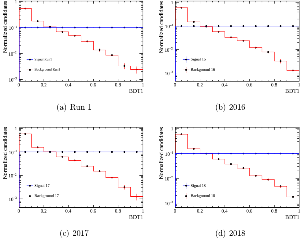
Figure A.9: Selection BDT distribution for 3\pi\mu signal and background training samples, using the Dalitz plane strategy. The flat transformation is applied.
