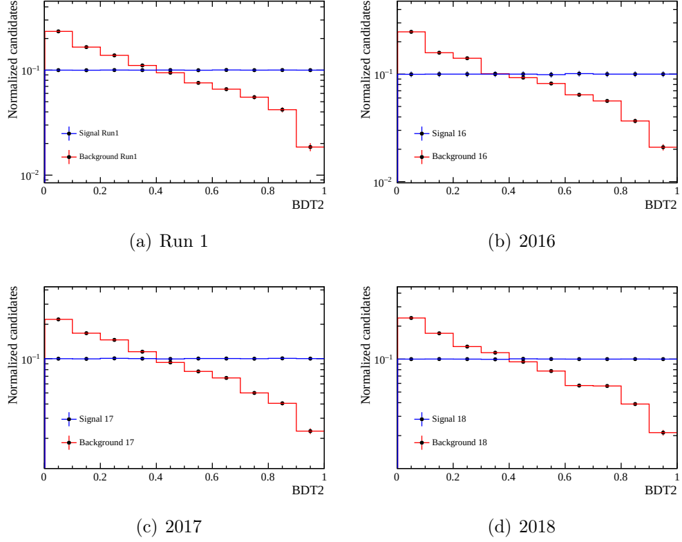
Figure 5.15: Distributions of BDT2 for 3\pi\mu signal and background training samples. The flat transformation is applied.
