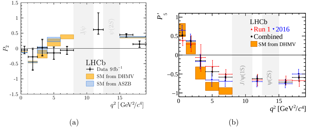
Figure 1.8: Experimental measurements of the P_2 (a) and P_5' (b) observables for the B^+ \rightarrow K^{*+} \mu^+ \mu^- and B^0 \rightarrow K^{*0} \mu^+ \mu^- analyses respectively.
