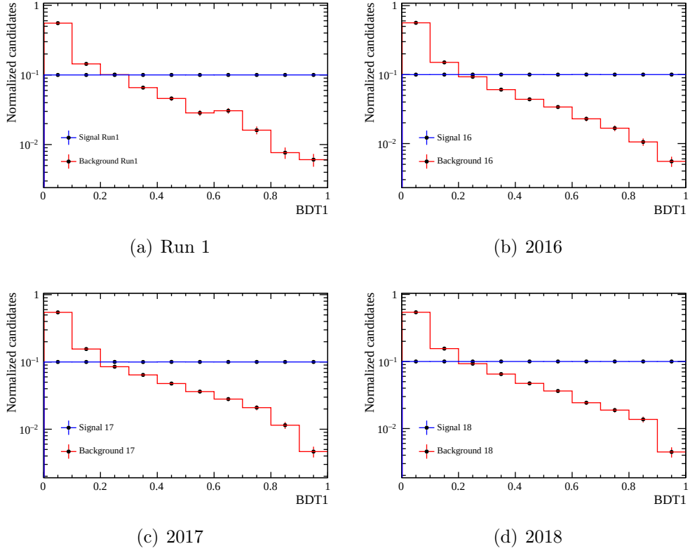
Figure 5.14: Distributions of BDT1 for 3\pi\mu signal and background training samples. The flat transformation is applied.
