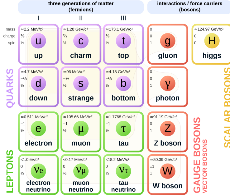
Figure 1.1: Elementary particles in the SM with some properties [19].
