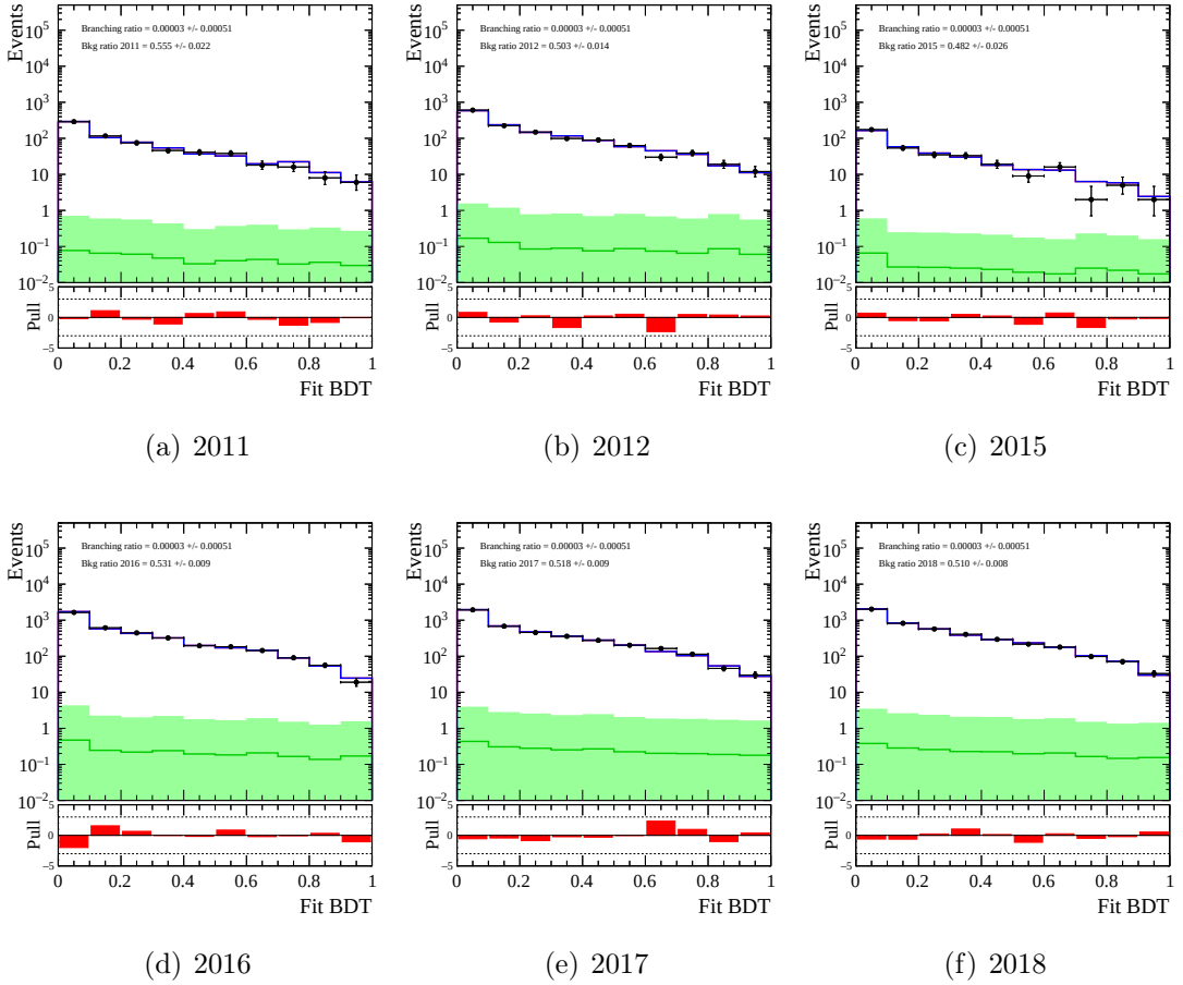
Figure 8.7: Result of the likelihood fit on a single toy experiment generated with initial signal branching ratio set to 0 for the 3\pi 3\pi final state. Shown are the generated data (black points), the signal (green), the background (red) and the total PDF (blue). The dashed lines in the pull correspond to the \pm 3\sigma difference.
