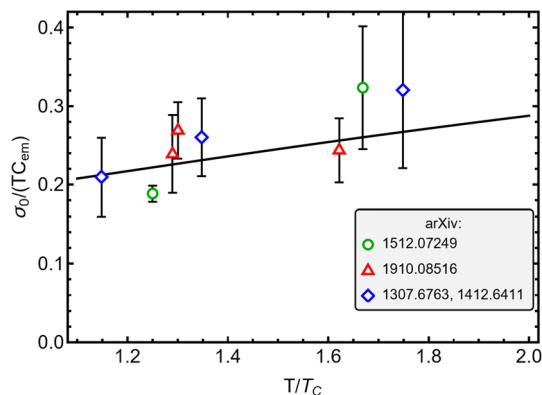
Fig. 20 The static conductivity \sigma_0 scaled with T as a function of temperature T scaled with the ‘critical’ value T_c \simeq 150 MeV as predicted by Eq. (2.64). ‘Experimental’ data are lattice results adapted from [107] for T > T_c . We indicate each set of points by its arXiv reference: blue diamonds [108, 109], green circles [110], and red triangles [111]. Adapted from Ref. [3]
