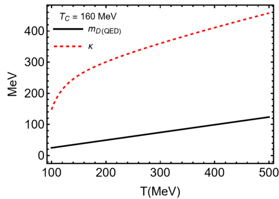
Fig. 19 The electromagnetic Debye mass m_D , solid (black) line, and the QCD damping rate \kappa , dashed (red) line, as a function of temperature. Published in Ref. [89] under the CC BY 4.0 license
