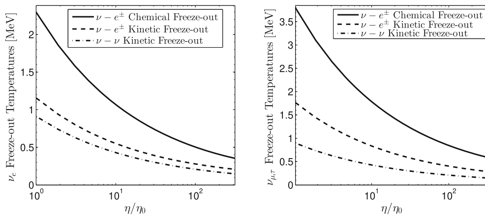
Fig. 6 Freeze-out temperatures for electron neutrinos (left-hand frame) and \mu, \tau neutrinos (right-hand frame) for the three types of processes, see insert, as functions of interaction strength \eta > \eta_0 . Published in Ref. [46] under the CC BY 4.0 license
