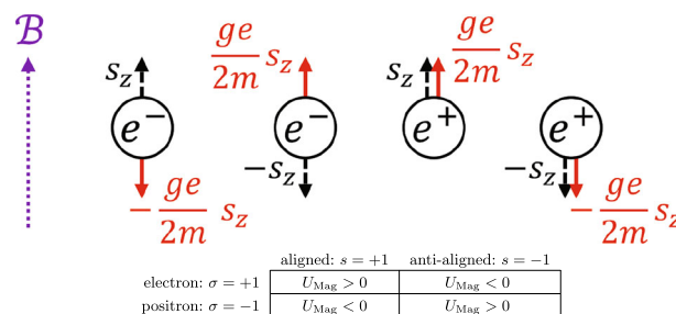
Fig. 56 Organizational schematic of matter-antimatter ( \sigma ) and polarization ( s ) states with respect to the sign of the nonrelativistic magnetic dipole energy U_{\text{Mag}} obtainable from Eq. (6.4). Published in Ref. [12] under the CC BY 4.0 license
