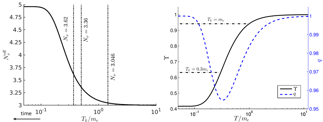
Fig. 28 Dependence of the effective number of neutrinos (left-hand frame) and neutrino fugacity (right-hand frame) on the neutrino kinetic freeze-out temperature. We also show the evolution of the deceleration parameter through the freeze-out period (right-hand frame)
