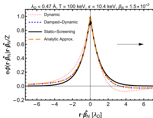
Fig. 52 Total screening potential scaled with charge Z and distance along the direction of motion. We show a comparison of the following screening models plotted along the direction of motion of a nucleus \mathbf{r} \cdot \hat{\beta}_N : static screening (black), dynamic screening (red dotted) from [239], damped-dynamic screening (blue dashed), and the approximate analytic solution of Eq. (5.93) (orange dashed). A black arrow indicates the direction of motion of the nucleus \hat{\beta}_N . Published in Ref. [217] under the CC BY 4.0 license
