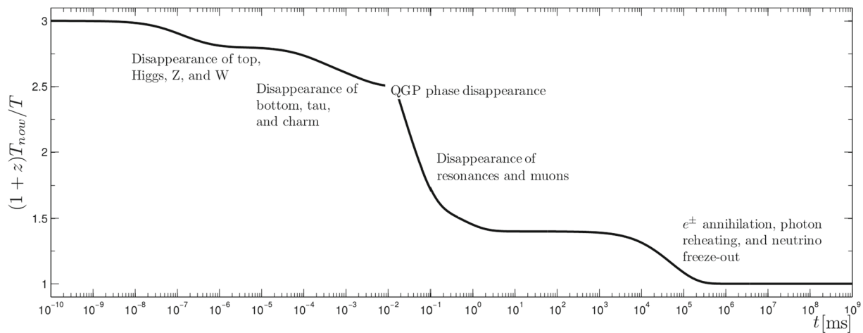
Fig. 10 Universe inflation due to the disappearance of degrees of freedom as a function of time t [ms] (milliseconds). The Universe volume inflated by approximately a factor of 27 above the naive thermal redshift scale as massive particles disappeared successively from the inventory while entropy remained conserved. Adapted from Ref. [2]
