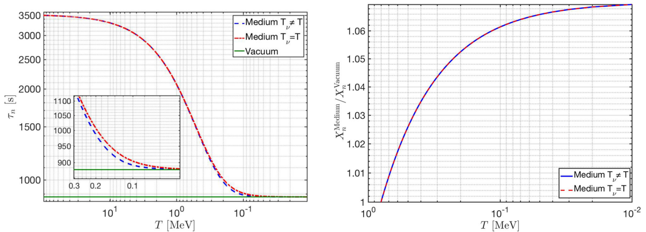
Fig. 50 On left: the neutron lifetime \tau_n^{\text{Medium}} in the cosmic plasma; On right: the neutron abundance ratio to vacuum abundance, as a function of temperature. Published in Ref. [233] under the CC BY 4.0 license
