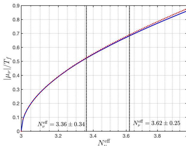
Fig. 35 The free-streaming neutrino chemical potential |\mu_\nu|/T_f as a function of the effective number of neutrinos N_\nu^{\text{eff}} . The solid (blue) line is the exact solution and the (red) dashed line is the approximate solution neglecting the (\mu_\nu/T_f)^4 term; the maximum difference in the domain shown is about 2%. Adapted from Ref. [5]
