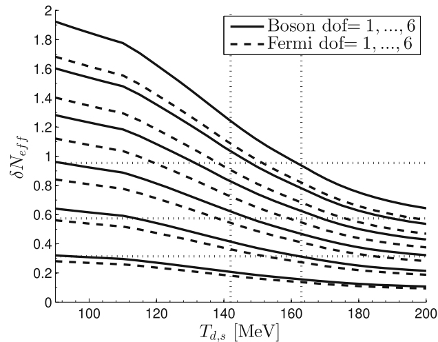
Fig. 30 Solid lines: increase in \delta N_{\text{eff}} due to the effect of 1, ..., 6 light sterile boson DoF ( g_s = 1, \dots, 6 , bottom to top curves) as a function of freeze-out temperature T_{d,s} . Dashed lines: increase in \delta N_{\text{eff}} due to the effect of 1, ..., 6 light sterile fermion DoF ( g_s = 7/8 \times 1, \dots, 7/8 \times 6 , bottom to top curves) as a function of freeze-out temperature T_{d,s} . The horizontal dotted lines correspond to \delta N_{\text{eff}} + 0.046 = 0.36, 0.62, 1 . The vertical dotted lines show the reported range of QGP transformation temperatures T_c = 142 - 163 MeV. Published in Ref. [137] under the CC BY 4.0 license
