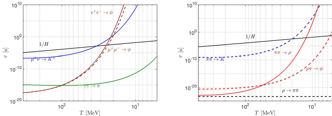
Fig. 26 Hadronic relaxation reaction times, see Eq. (2.89), as a function of temperature T , are compared to Hubble time 1/H (black solid line). On right the bottom horizontal black-dashed line is the natural (vacuum) lifespan of \rho . Published in Ref. [1] under the CC BY 4.0 license. Adapted from Ref. [5, 10]
