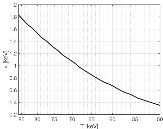
Fig. 49 The relaxation rate \kappa that satisfies Eq. (5.43) self-consistently as a function of temperature 50 \leq T \leq 86 \text{ keV} . The minor fluctuations are due to limited numerical precision. Adapted from Ref. [5]
