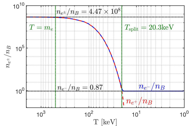
Fig. 55 Number density of electron e^- and positron e^+ to baryon ratio n_{e^\pm}/n_B as a function of photon temperature in the primordial Universe. See Sect. 5.2 for further details. In this work we measure temperature in units of energy (keV) thus we set the Boltzmann constant to k_B = 1 . Published in Ref. [12] under the CC BY 4.0 license
