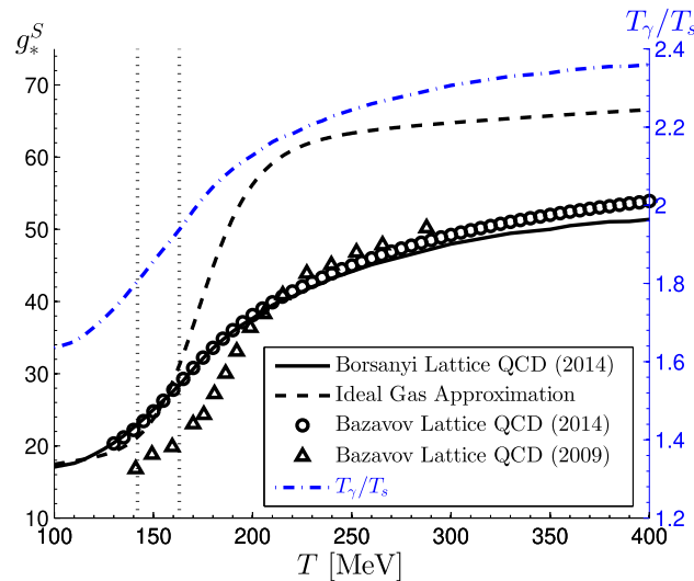
Fig. 29 Left axis: effective number of entropy-DoF, including lattice QCD effects applying [52] (solid line) and [146] (circles), compared to the earlier results [147] (triangles) used by [144], and the ideal gas model of [148] (dashed line) as functions of temperature T . Right axis: photon to SP temperature ratio, T_\gamma/T_s , as a function of SP decoupling temperature (dash-dotted (blue) line). The vertical dotted lines at T = 142 MeV and T = 163 MeV delimit the QGP transformation region. Published in Ref. [137] under the CC BY 4.0 license
