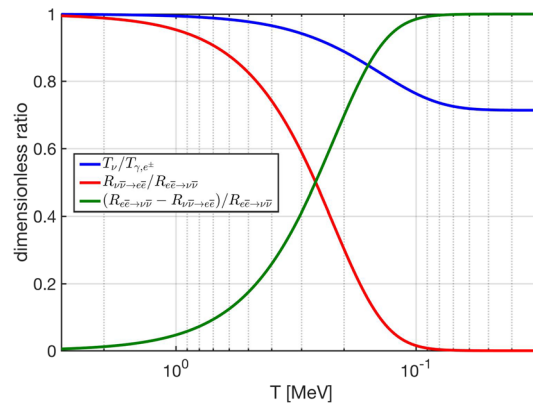
Fig. 38 The temperature ratio T_\nu/T_{\gamma, e^\pm} (blue line), the rate ratio R_{\nu\bar{\nu} \rightarrow e\bar{e}}/R_{e\bar{e} \rightarrow \nu\bar{\nu}} (red line) and (R_{e\bar{e} \rightarrow \nu\bar{\nu}} - R_{\nu\bar{\nu} \rightarrow e\bar{e}})/R_{e\bar{e} \rightarrow \nu\bar{\nu}} (green line) as a function of temperature. It shows that the reaction \nu\bar{\nu} \rightarrow e\bar{e} is small compare to the reaction e\bar{e} \rightarrow \nu\bar{\nu} as temperature cooling down. Adapted from Ref. [5]
