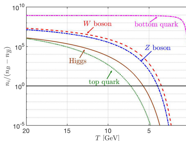
Fig. 11 The ratio between thermal equilibrium density of heavy particles t, h, Z, W, b with the baryon excess density n_B - n_{\bar{B}} as a function of temperature 20 \text{ GeV} > T > 0.1 \text{ GeV} . Adapted from Ref. [5]
