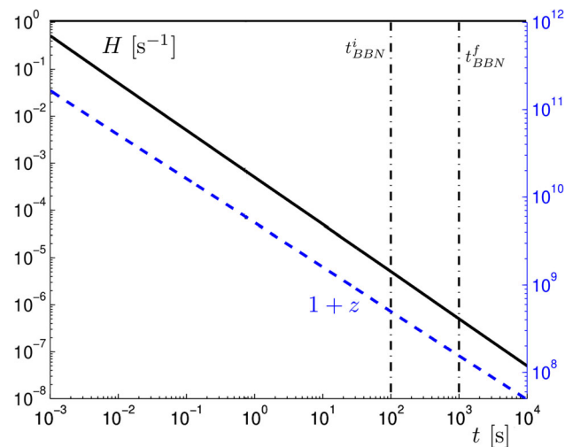
Fig. 9 First hours in the evolution of the universe: Hubble parameter H in units [1/s] (left-hand scale) and the redshift 1+z (right-hand scale, blue) spanning the epoch from well below the end of baryon antimatter annihilation through BBN, compare Fig. 8. Adapted from Ref. [44]. Published in Ref. [46] under the CC BY 4.0 license
