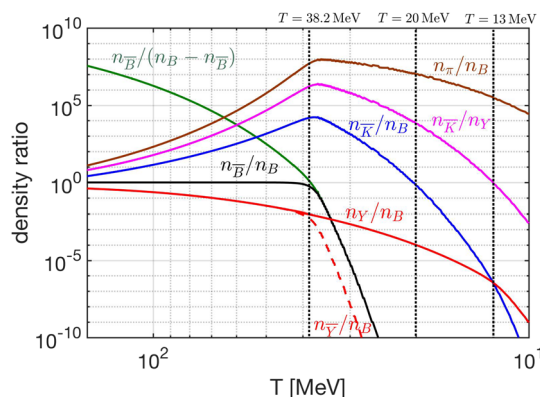
Fig. 24 Ratios of hadronic particle number densities with baryon B yields as a function of temperature 150 \text{ MeV} > T > 10 \text{ MeV} : pions \pi (brown line), kaons K(q\bar{s}) (blue), antibaryon \bar{B} (black), hyperon Y (red) and anti-hyperons \bar{Y} (dashed red). Also shown \bar{K}/Y (purple). Vertical lines highlight events described in text. Published in Ref. [1] under the CC BY 4.0 license. Adapted from Ref. [10]
