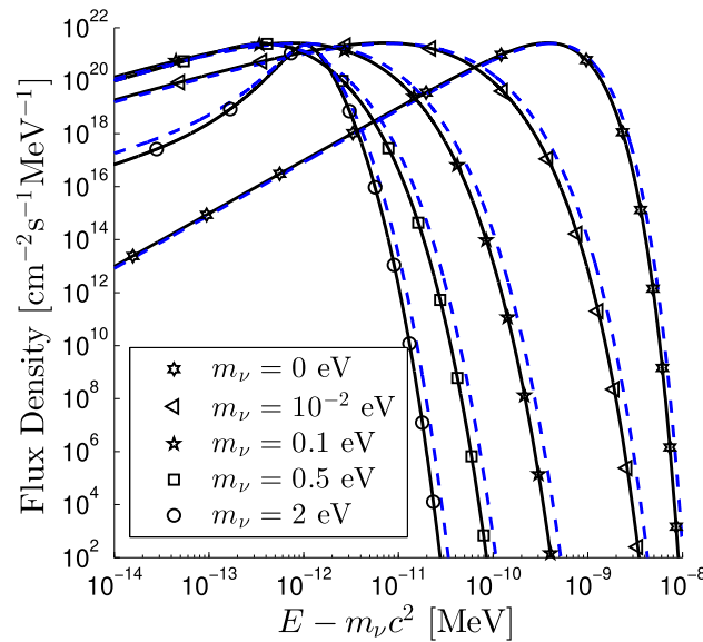
Fig. 41 Neutrino flux density in the Earth frame. We show the result for N_\nu^{\text{eff}} = 3.046 (solid lines) and N_\nu^{\text{eff}} = 3.62 (dashed lines) for an observer moving with v_\oplus = 300 km/s. Published in Ref. [167] under the CC BY 4.0 license
