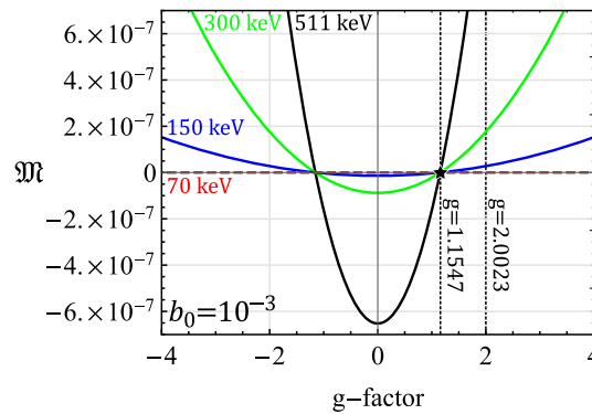
Fig. 59 The magnetization \mathfrak{M} as a function of g -factor plotted for several temperatures with magnetic scale b_0 = 10^{-3} and polarization fugacity \xi = 1 . Published in Ref. [4] under the CC BY 4.0 license. Adapted from Ref. [12]
