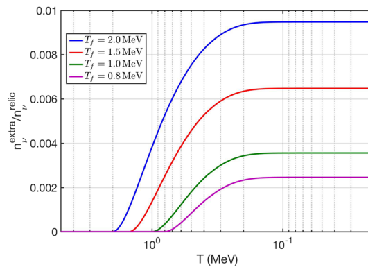
Fig. 39 The ratio between n_{extra}/n_{relic} as a function of temperature with different neutrino freeze-out temperature T_f . Adapted from Ref. [5]
