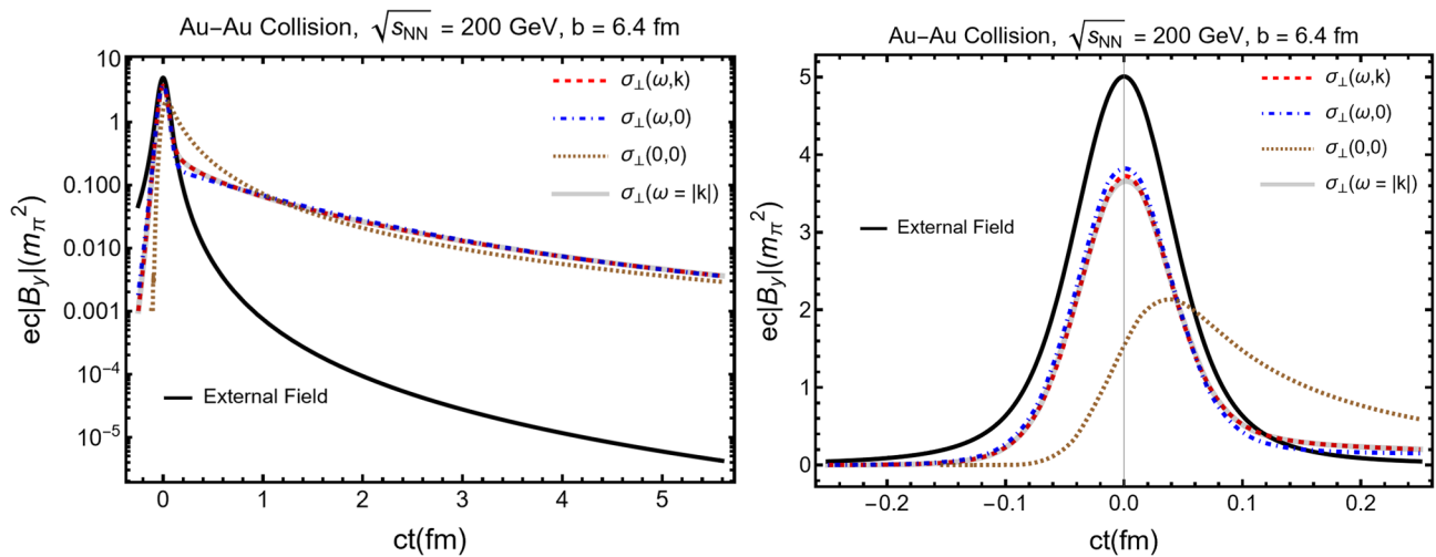
Fig. 21 The magnetic field at the collision center as a function of time, for QGP at T = 300 MeV formed in Au–Au collisions ( Z = 79 ) at \sqrt{s_{\text{NN}}} = 200 GeV and impact parameter b = 6.4 fm. The left-hand frame shows the magnetic field on a semi-logarithmic scale up to ct = 5 fm. The right-hand frame shows the early-time magnetic field on a linear scale. Published in Ref. [89] under the CC BY 4.0 license
