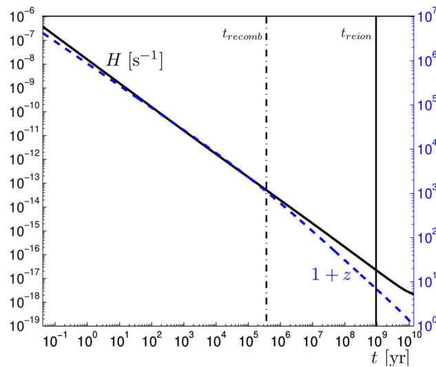
Fig. 4 Temporal evolution of the Hubble parameter H (in units 1/s ) (left-hand scale) and of redshift 1 + z (right-hand scale, blue). Adapted from Ref. [44]
