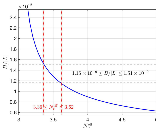
Fig. 36 The ratio B/|L| between the net baryon number and the net lepton number as a function of N_\nu^{\text{eff}} : The solid blue line shows B/|L| . The vertical (red) dotted lines represent the values 3.36 \leq N_\nu^{\text{eff}} \leq 3.62 , which correspond to 1.16 \times 10^{-9} \leq B/|L| \leq 1.51 \times 10^{-9} (horizontal dashed lines). Adapted from Ref. [5]
