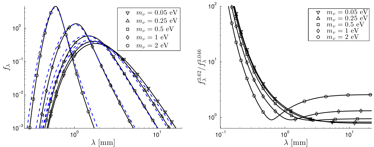
Fig. 42 Neutrino FDEV de Broglie wavelength distribution in the Earth frame. We show in left panel the distribution for N_\nu^{\text{eff}} = 3.046 (solid lines) and N_\nu^{\text{eff}} = 3.62 (dashed lines) and in right panel their ratio. Published in Ref. [167] under the CC BY 4.0 license
