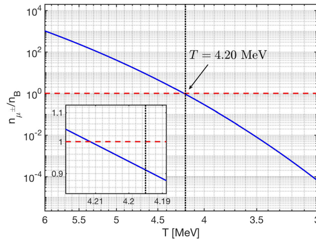
Fig. 45 The density ratio between \mu^\pm and baryons as a function of temperature. The density ratio at muon disappearance temperature is n_{\mu^\pm}/n_B(T_{\text{disappear}}) \approx 0.911 , and around the temperature T \approx 4.212 MeV the computed density ratio n_{\mu^\pm}/n_B \approx 1 . Published in Ref. [1] under the CC BY 4.0 license. Adapted from Ref. [5, 116]
