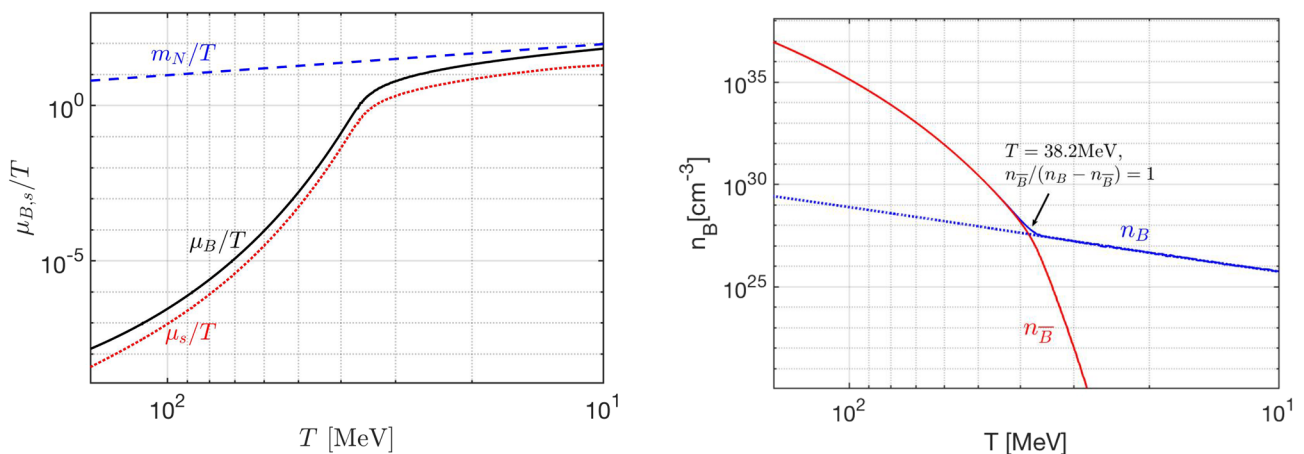
Fig. 23 Left frame: solid (black) line baryon number chemical potential \mu_B/T ; dotted (red) line strangeness chemical potential \mu_s/T , as a function of temperature 150 \text{ MeV} > T > 10 \text{ MeV} in the primordial Universe; for comparison we show dashed (blue) m_N/T with m_N = 938.92 \text{ MeV} , the average nucleon mass. Published in Ref. [10] under the CC BY 4.0 license. Adapted from Ref. [5] Right frame: Net baryon number n_B - n_{\bar{B}} in the temperature range 150 \text{ MeV} > T > 5 \text{ MeV} , the dashed (blue) line turns into solid (blue) line depicting baryon density n_B once the antibaryon n_{\bar{B}} number density, solid line (red), diminishes; the transition point n_{\bar{B}}/(n_B - n_{\bar{B}}) = 1 is at T = 38.2 \text{ MeV} . Published in Ref. [1] under the CC BY 4.0 license. Adapted from Ref. [5]
