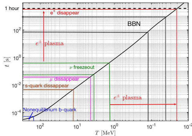
Fig. 5 The relation between time and temperature in the first hour of the Universe beginning shortly before QGP hadronization 300 \text{ MeV} > T > 0.02 \text{ MeV} and ending with antimatter disappearance. Temperature/time range for several epochs is indicated. Adapted from Ref. [5]
