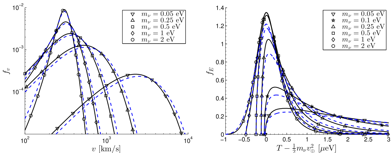
Fig. 40 Normalized neutrino FDEV for velocity on left and energy on right. We show the distribution for N_\nu^{\text{eff}} = 3.046 (solid lines) and N_\nu^{\text{eff}} = 3.62 (dashed lines). Published in Ref. [167] under the CC BY 4.0 license
