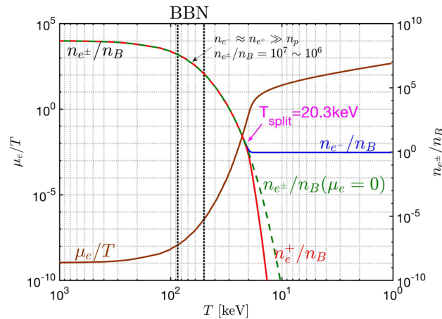
Fig. 46 Left axis: the chemical potential of electrons \mu_e/T as a function of temperature (solid (brown) line). Right axis: the ratio of electron (positron) number density to baryon density as a function of temperature. The solid blue line is the electron density, the red line is the positron density, and the green dashed line is obtained setting for comparison \mu_e = 0 . The vertical black dotted lines are bounds of BBN epoch. Published in Ref. [217] under the CC BY 4.0 license. Adapted from Ref. [5]
