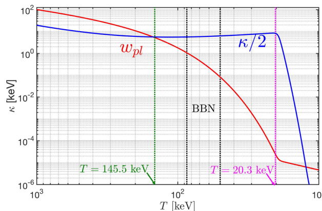
Fig. 48 The relaxation rate \kappa/2 (blue line) and plasma frequency \omega_{\text{pl}} (red line) as a function of temperature in non-relativistic electron-positron plasma. Vertical green dashed line indicates the boundary between over- and under-damped plasma at T < 145.5 keV which is before the BBN epoch (vertical black lines). Temperature domain of validity is above disappearance of positrons (vertical line at 20.3 keV). Adapted from Ref. [5]
