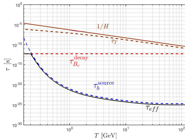
Fig. 16 The effective relaxation time \tau_{\text{eff}} as a function of temperature in the primordial Universe for bottom mass m_b = 4.7 GeV. For comparison, we also plot the vacuum lifespan of B_c meson \tau_{B_c}^{\text{decay}} (red dashed-line), the relaxation time for bottom production \tau_{\text{source}}^b (blue dashed-line), Hubble expansion time 1/H (brown solid line) and relaxation time for temperature cooling \tau_T (brown dashed-line). Adapted from Ref. [5]
