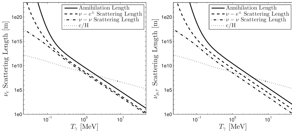
Fig. 31 Comparison of Hubble parameter to neutrino scattering length for various types of PP-SM processes, left-hand frame for electron neutrino \nu_e and right-hand frame for the other two flavors \nu_\mu , \nu_\tau . Published in Ref. [46] under the CC BY 4.0 license
