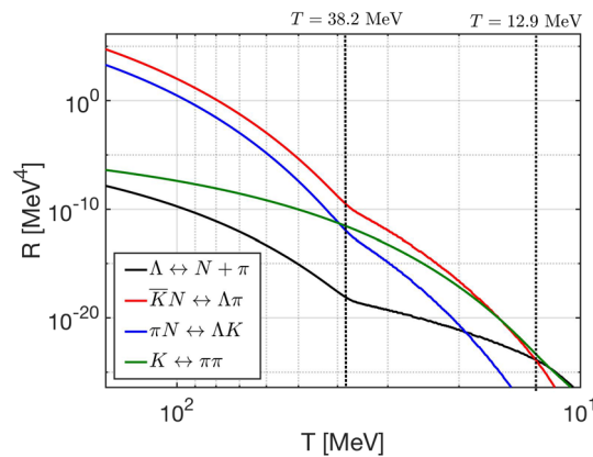
Fig. 27 Thermal reaction rate R per volume and time for important hadronic strangeness production and exchange processes as a function of temperature 150 \text{ MeV} > T > 10 \text{ MeV} in the primordial Universe. Published in Ref. [1] under the CC BY 4.0 license. Adapted from Ref. [5, 10]
