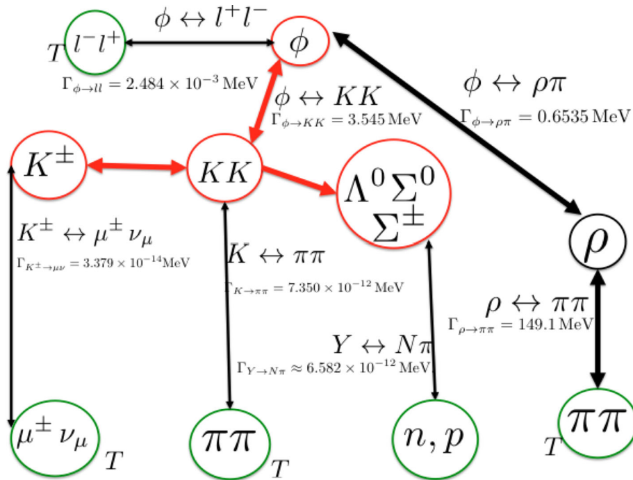
Fig. 25 The strangeness abundance changing reactions in the primordial Universe. The central circles (red) show strangeness carrying hadronic particles; red thick lines denote effectively instantaneous reactions. Black thick lines show relatively strong hadronic reactions. Published in Ref. [1] under the CC BY 4.0 license. Adapted from Ref. [5, 10]
