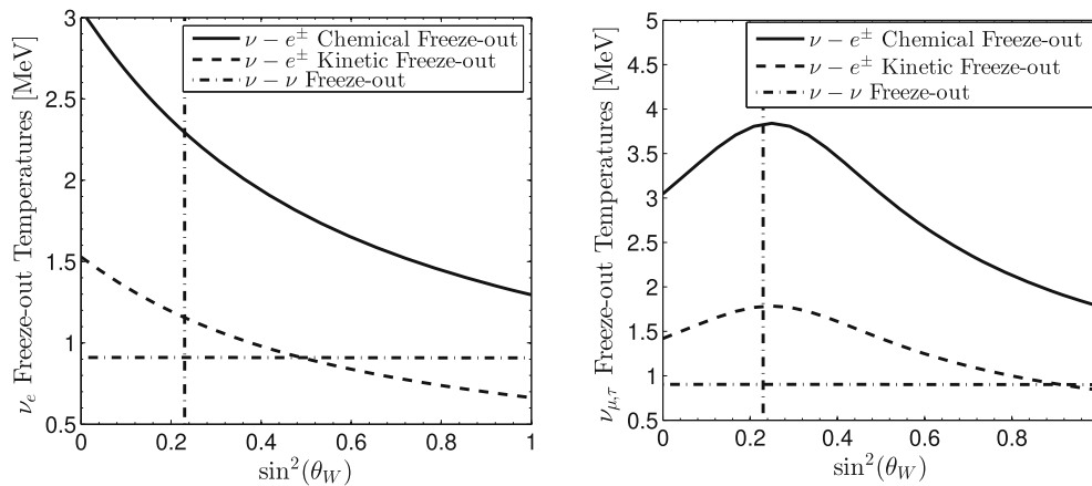
Fig. 7 Freeze-out temperatures for electron neutrinos (left-hand frame) and \mu, \tau neutrinos (right-hand frame) for three types of processes, see insert, as functions of the value of the Weinberg angle \sin^2(\theta_W) . Vertical line is at present epoch \sin^2(\theta_W) = 0.23 . Published in Ref. [46] under the CC BY 4.0 license
