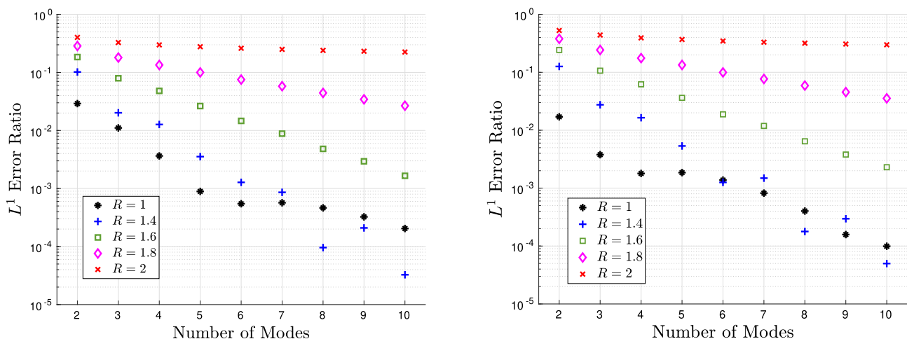
Fig. 63 Errors in expansion of Eq. (C.32) as a function of number of modes, left-hand side for \mathcal{R} = 0.5 and right-hand side for \mathcal{R} = 1.5 . Adapted from Ref. [30]
