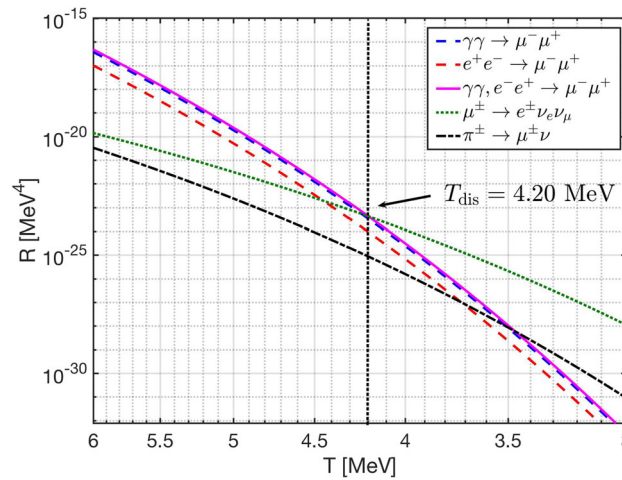
Fig. 44 The thermal reaction rate per time and volume for different muon reactions as a function of temperature. See text. Published in Ref. [1] under the CC BY 4.0 license. Adapted from Ref. [5, 116]
