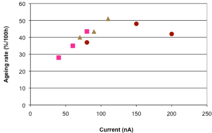
Fig. 6 Aging rate in the TRT straws as a function of the current density (nA in 1 cm of irradiated wire).
