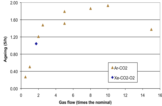
Fig. 5 Aging rate in the TRT straws as function of gas flow, expressed as times the nominal LHC flow of one volume exchange per hour.
