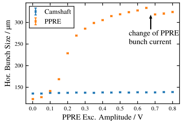
Figure 3: Measured horizontal size of the PPRE and the camshaft bunch as a function of the PPRE excitation amplitude.
