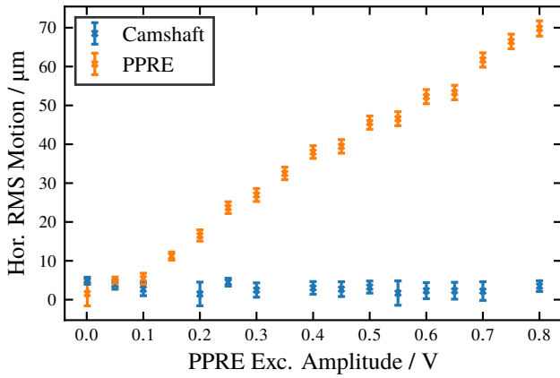
Figure 4: Measured horizontal orbit motion of the PPRE and the camshaft bunch as a function of the PPRE excitation amplitude.
