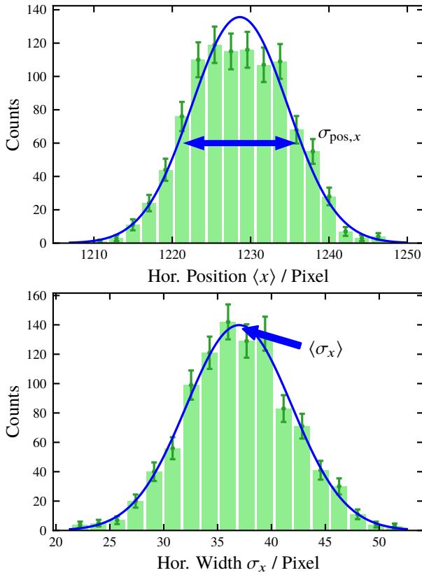
Figure 2: Histogram of the measured horizontal position (top) and the horizontal width (bottom) of the PPRE bunch from 1000 single-shot streak camera images. Additionally a Gaussian given by the mean and standard deviation of the distributions is shown.
