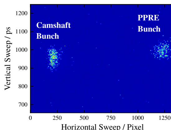
Figure 1: Single-shot single-turn streak camera measurement from the camshaft and the PPRE bunch at the new diagnostics beamline.
