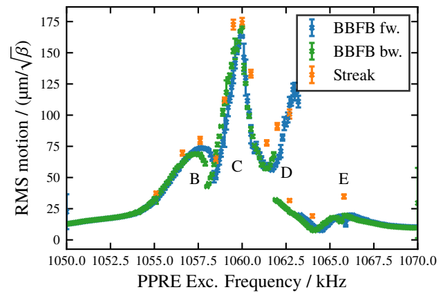
Figure 7: Horizontal PPRE bunch motion measured with the streak camera and the BBFB system (for two scanning directions) as a function of the PPRE excitation frequency, normalized by the horizontal \beta -function at respective source points.
