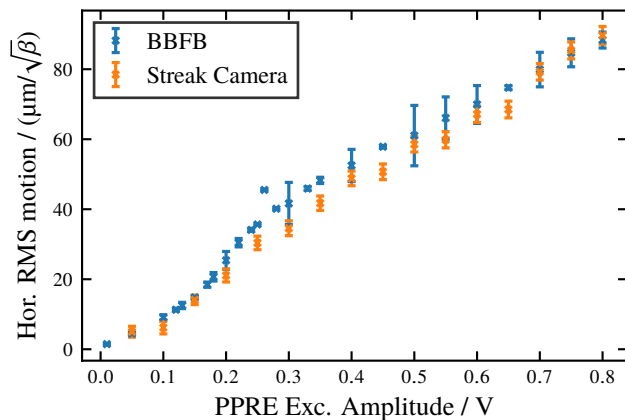
Figure 5: Horizontal PPRE bunch motion measured with the streak camera and the BBFB system as a function of the PPRE excitation amplitude, normalized by the horizontal \beta -function at respective source points.
