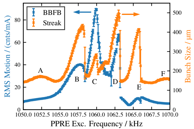
Figure 6: Horizontal size of the PPRE bunch measured with the streak camera and PPRE bunch motion measured with the BBFB system as function of the excitation frequency.
