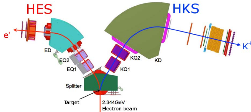
Figure 1. Plan view of the high-resolution kaon spectrometer (HKS) and a new high-resolution electron spectrometer (HES) for the E05-115 experiment.
