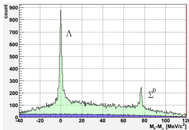
Figure 3. Missing mass spectrum for CH 2 target with a subtraction of \Lambda 's mass. Accidental background is shown as hatched region. Remaining events under hyperon peaks are originating from quasi-free hyperon production from carbon.
