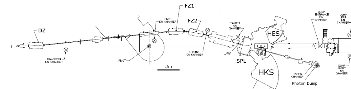
Figure 2. Pre-chicane beamline newly constructed in JLab Hall-C.
