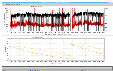
Figure 5: The upper plot shows the fixed target event rate (in black) and min-bias rate (in red) over the time period of two physics stores at 13.5 GeV. The lower plot shows the beam intensity evolution during the stores, total beam intensity in light yellow and bunched beam intensity in dark yellow.
