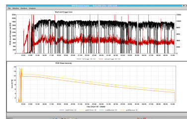
Figure 4: The upper plot shows the fixed target event rate (in black) and min-bias rate (in red) over the time period of a physics store at 19.5 GeV/n. The lower plot shows the beam intensity evolution during the store, total beam intensity in light yellow and bunched beam intensity in dark yellow.
