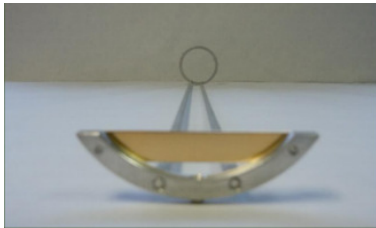
Figure 1: Picture of the STAR gold fixed target. The target was inserted in the lower part of the beam pipe.
