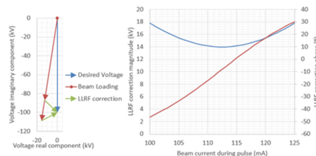
Figure 4: Beam loading and LLRF correction for a desired cavity bunching voltage of 100 kV and beam current between 100 and 125 mA. Complex representation (left). Amplitude and phase of the correction as a function of the beam current(right).
