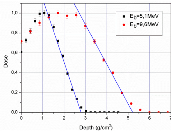
Figure 4: Measured dose - depth distribution in Al. Set energies are 5 MeV and 10 MeV.
