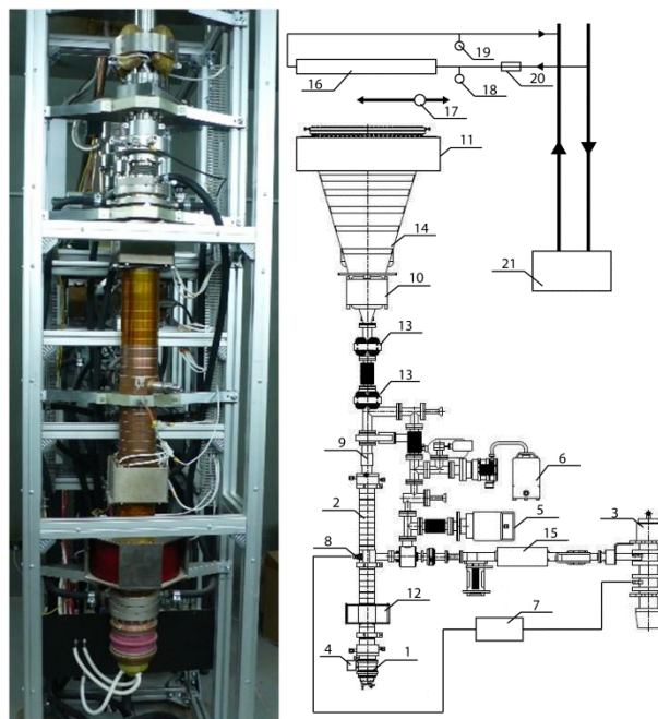
Figure 1: Photo and schematic view of the accelerator. 1 – electron gun, 2 – accelerating structure, 3 – klystron, 4, 5, 6 – vacuum pumps, 7 – low power RF unit, 8 – RF antenna, 9 – beam current monitor, 10 – scanning magnet, 11 – correcting magnet, 12 – solenoid, 13 – quadrupole lenses, 14 – scanning chamber, 15 – circulator, 16 – beam absorber 1, 17 – beam absorber 2, 18, 19 – temperature sensors, 20 – flow meter, 21 – chiller.
