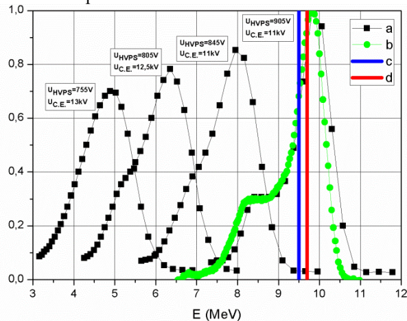
Figure 5: The beam spectra measured by the absorber 16 (Fig. 1) (a), by radiochromic film (b), beam energy from dose-depth distribution measurement (c) and from average power and pulsed current measurements (d).
