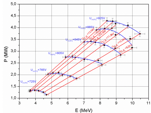
Figure 3: The relation of pulsed beam power and beam energy for the selected operation mode of the accelerator. U_{HVPS} is the charging voltage of modulator, U_{CE} is the electron gun control electrode voltage.
