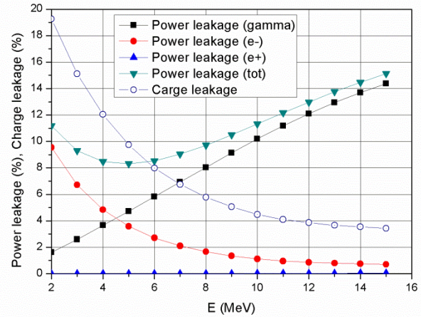
Figure 2: The dependence of the beam power and charge leakage on the electron energy due to the bremsstrahlung, secondary electrons and positrons.
