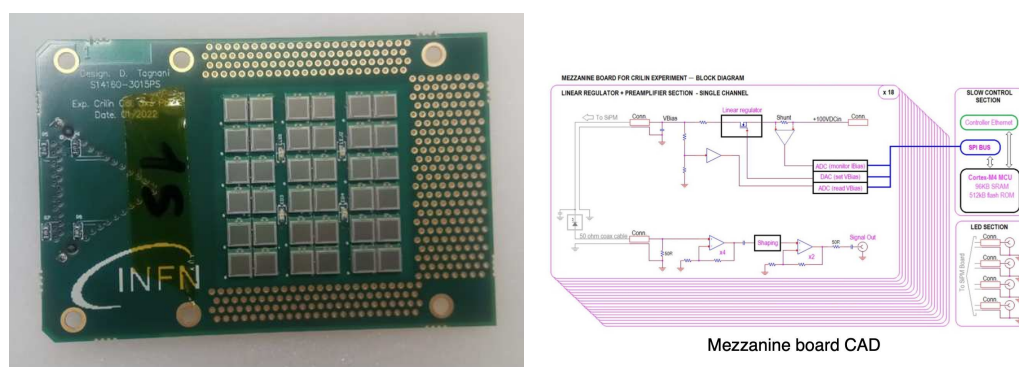
Figure 8. (Left): SiPMs board detail, showing the sensor matrices and the LEDs. (Right): Mezzanine Boards CAD rendering.
