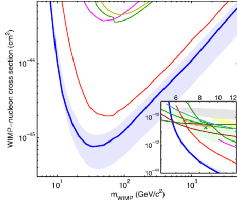
Figure 2: 90% Confidence limits on WIMP nucleon scattering from LUX Run 3 data, Blue (line and band) LUX 2013 result 10) . For comparison, we include limits from: XENON100 (red), ZEPLINIII (magenta), CDMSII (green) and EDELWEISSII (dark yellow). The inset shows limits and results for WIMP nucleon scattering at low mass. The low mass region also includes results (closed regions) from: CoGeNT (orange), CDMSII-Si (green), CRESSTII (yellow), and DAMA-LIBRA (grey).
