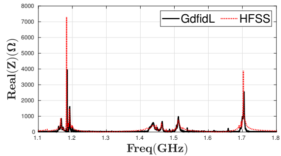
Figure 5: Longitudinal impedance as from GdfidL and HFSS.
