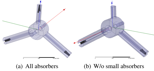
Figure 2: 3D Models for GdfidL, in brown the ferrite loads.
