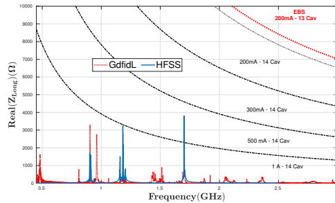
Figure 7: Longitudinal Impedance without the small damper and with all the ancillaries (IP and tuner).
