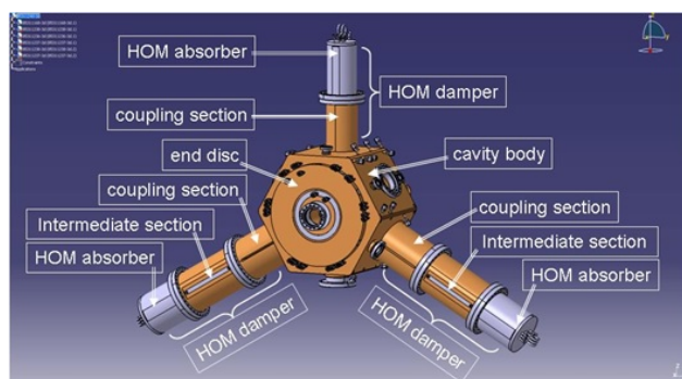
Figure 1: Overview of the main components of the ESRF-EBS cavity.
