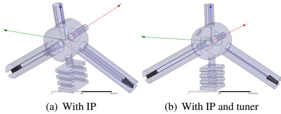
Figure 3: 3D Models for GdfidL including the ancillaries, in brown the ferrite loads.
