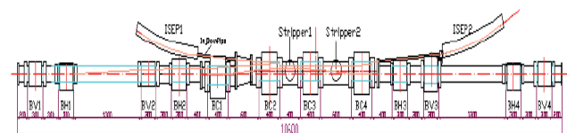
Figure 6: Machine layout of CSNS injection system.
