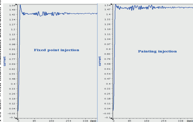
Figure 3: RCS DCCT displays while the fixed point injection and the painting injection were used.
