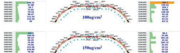
Figure 5: Different injection beam loss while the main stripping foils with different thicknesses.
