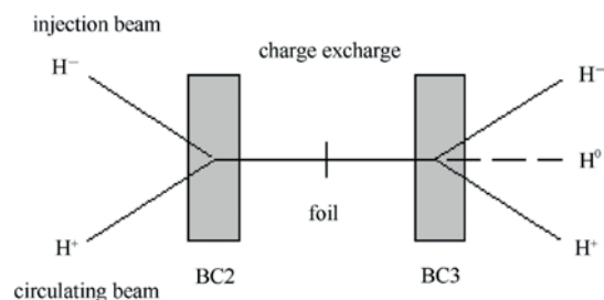
Figure 2: Production of H^- , H^0 and H^+ by foil stripping.
