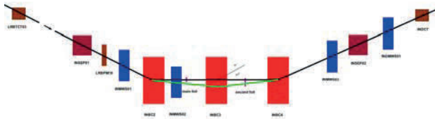
Figure 7: Physics design layout of the I-Dump beam line. The beam path with black colour is for the normal operation mode and the beam path with green colour is for the I-Dump operation mode.
