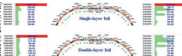
Figure 4: Different injection beam loss while the single-layer foil and double-layer foil were used.
