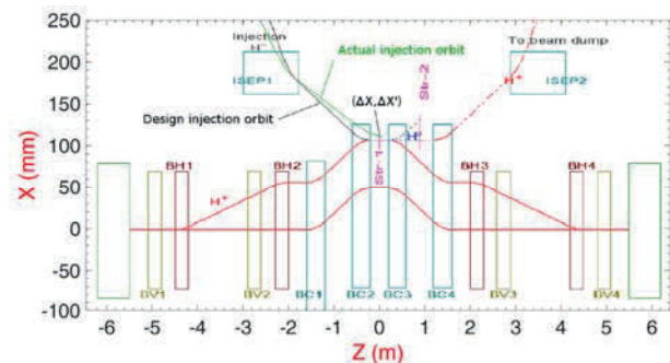
Figure 1: Physics design layout of CSNS injection system.
