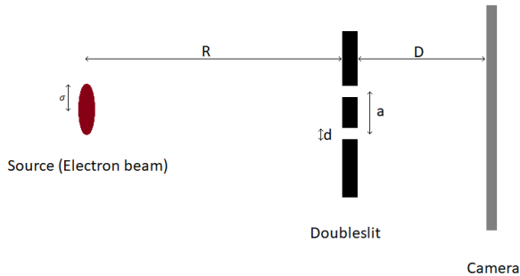
Figure 1: Double slit layout.
