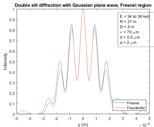
Figure 2: Typical intensity distribution.
