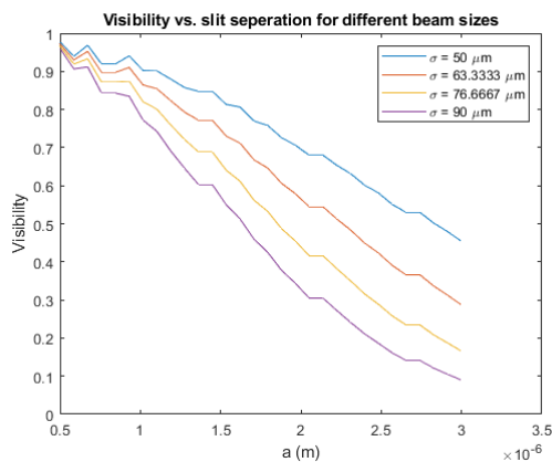
Figure 3: Visibility versus slit separation.
