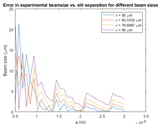
Figure 4: Error versus slit separation.
