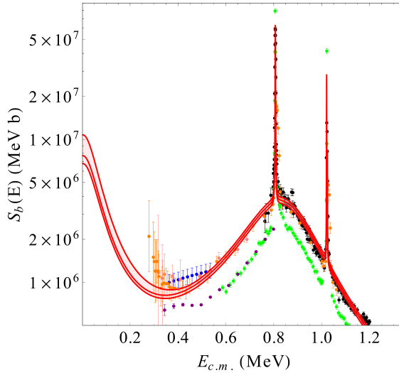
Fig. 2. (Colour on-line) R-matrix astrophysical factor (central/red curve) calculated adopting the resonance deduced from the THM cross section using Eq. (2). Normalisation and statistical uncertainties (including correlations) are given by the lower and upper red lines. Direct data, reported without any scaling, are shown as symbols [35, 41–45].
