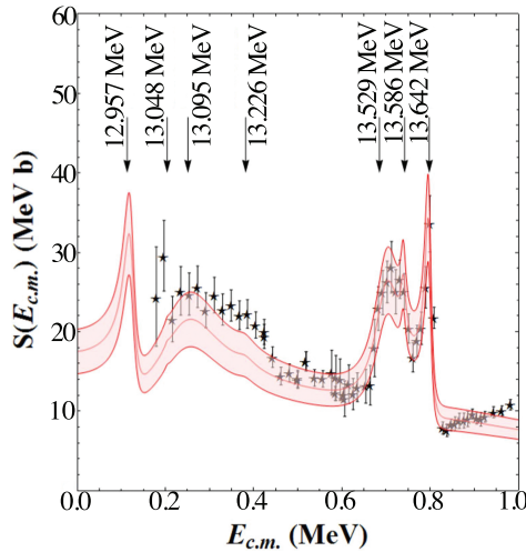
Fig. 3. (Colour on-line) Comparison of the THM S -factor with direct data. The THM result is shown as a grey/red band, highlighting the upper and lower limits allowed for by the normalisation and statistical errors. The black stars represent the experimental data from Refs. [49, 53]. Finally, the arrows indicate the ^{20}\text{Ne} levels contributing to the S(E) -factor.
