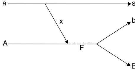
Fig. 1. Diagram illustrating the population of excited states of the intermediate system F via a QF mechanism, proceeding through the direct break up of the TH nucleus a and the capture of the participant cluster x by the target nucleus A .
