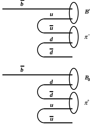
Figure 6-1: Possible fragmentation paths for a \bar{b} quark, assuming a naive view of string fragmentation.
