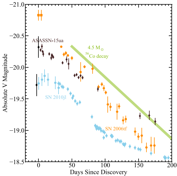
Figure 5. Absolute V -band magnitudes for IIn SLSNe: ASASSN-15ua, SN2006tf (Smith et al. 2008b), and SN2010jl (Stoll et al. 2011; Fransson et al. 2014). SN 2006tf and SN 2010jl have been adjusted to absolute magnitude adopting E(B - V) values and distances described in the text. The squares are the unfiltered discovery observations of SN 2006tf. A slope corresponding to the radioactive decay rate consistent with 4.5 M_{\odot} of ^{56}\text{Co} is shown for comparison.
