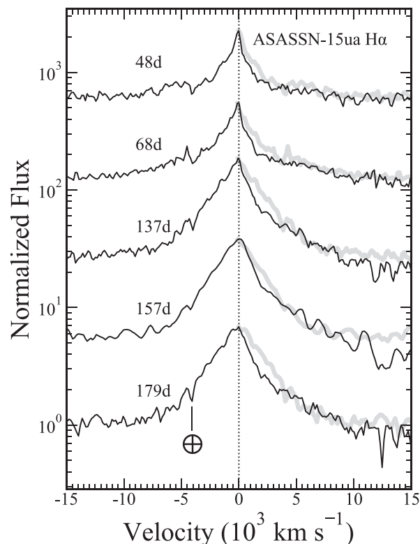
Figure 8. The same H \alpha line profiles as in Fig. 7 but separated vertically. This plot shows the blueshifted wing of the line reflected over (shown in a thicker line) to redshifted velocities. There is a consistent flux deficit on the observed redshifted wings, even though the narrow line peak is at zero velocity.
