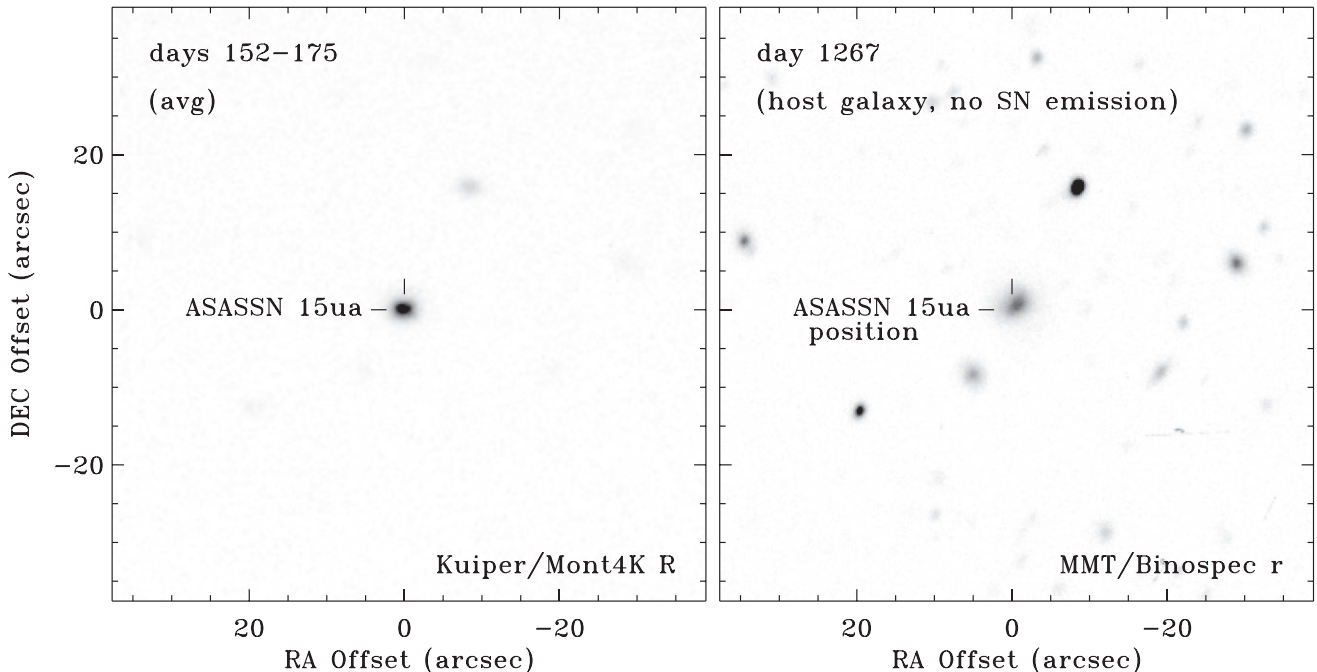
Figure 1. Images of the SN location with and without SN light. Left: Kuiper/Mont4k R -band image of ASASSN-15ua with the SN location identified. This is an average of three images taken between days 152 and 175 after discovery, when SN light still dominated the observed flux. Right: MMT/Binospec r -band image of the same field at late times after the SN faded, showing its location in its host galaxy GALEXASC J133454.49+105906.7 as measured in the Kuiper image in the left panel.
