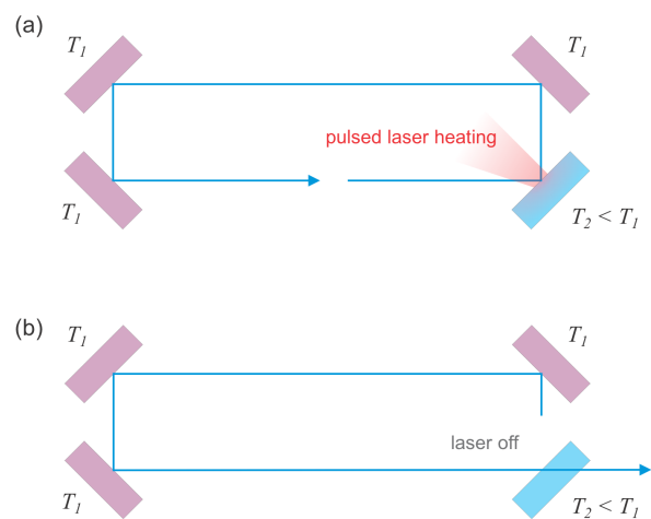
Figure 2: (a) Configuration of the closed cavity. The lower right crystal is kept at lower temperature. A synchronized laser pulse is used to control the surface temperature and lattice constant to meet the Bragg condition. (b) configuration of an open cavity with the laser switched OFF. The lower right crystal at lower temperature would thus become transparent to the ‘resonant’ wavelength.
