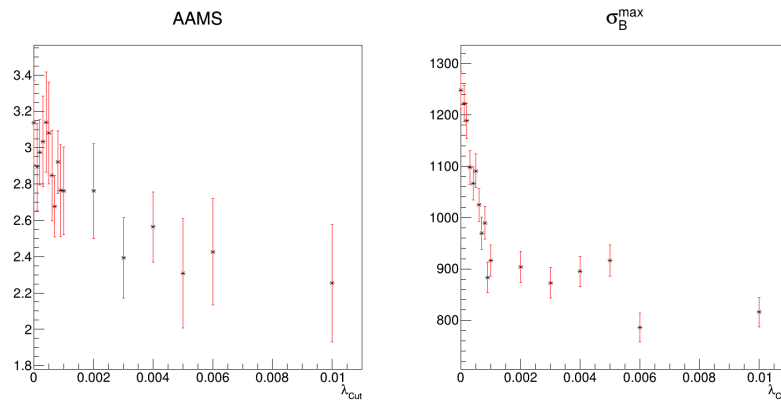
Figure 1. AAMS (left) and \sigma_B^{max} (right) for different values of \lambda_{Cut} .
