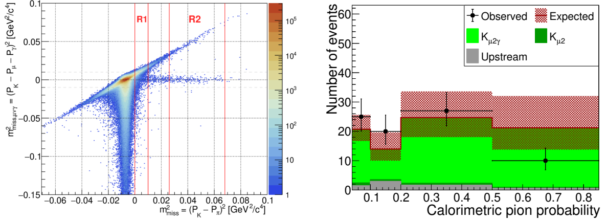
Figure 7. Left: event distribution in the (m^2_{\text{miss}}, m^2_{\text{miss}, \mu\nu\gamma}) plane for a minimum bias data control sample with MUV3 associated signals and no calorimetric BDT condition applied. The K^+ \rightarrow \mu^+ \nu \gamma candidates are clearly visible as a horizontal line around m^2_{\text{miss}, \mu\nu\gamma} = 0 extending towards high m^2_{\text{miss}} values including R2. Right: K^+ \rightarrow \mu^+ \nu \gamma background validation samples, four bins in sidebands of the calorimetric BDT pion probability. Expectations include contributions from K^+ \rightarrow \mu^+ \nu \gamma ( K_{\mu 2\gamma} ), K^+ \rightarrow \mu^+ \nu ( K_{\mu 2} ) and upstream (section 6.3) events.
