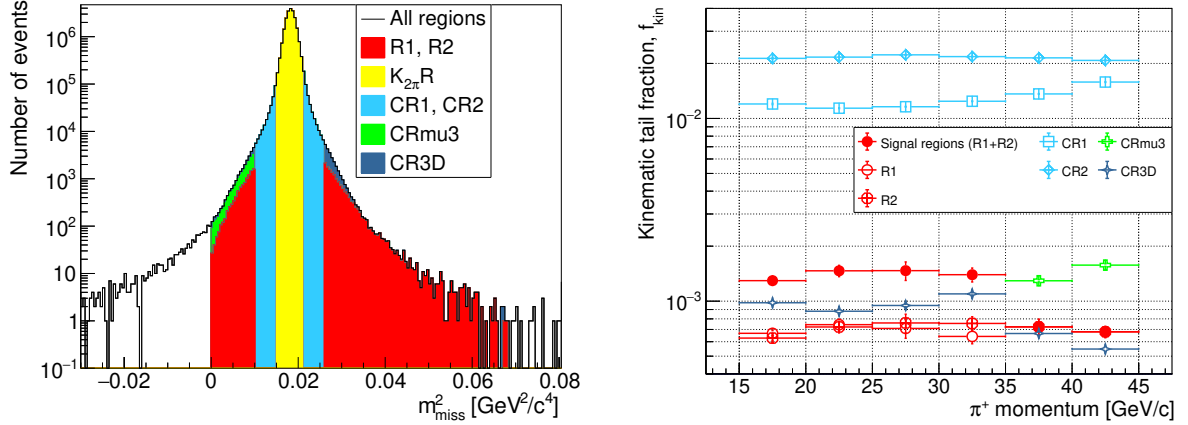
Figure 6. Left: distribution of m_{\text{miss}}^2 of the kinematic tails data control sample for K^+ \rightarrow \pi^+ \pi^0 decays. The colours show the contributions from the kinematic regions defined in figure 3-right. The average value of f_{\text{kin}}(K^+ \rightarrow \pi^+ \pi^0) is calculated as the ratio between the red area and the yellow area (and similarly for the control regions). Right: f_{\text{kin}}(K^+ \rightarrow \pi^+ \pi^0) as a function of the \pi^+ momentum, evaluated for signal regions (red) and for control regions (by exchanging the signal region with the corresponding control region).
