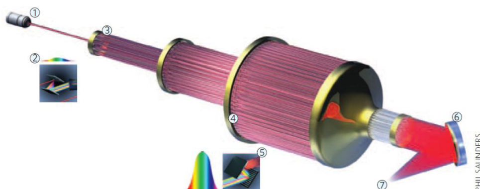
Fig. 2. Principle of a coherent amplifier network (CAN) based on fiber laser technology. An initial pulse from a seed laser (1) is stretched (2), and split into many fibre channels (3). Each channel is amplified in several stages, with the final stages producing pulses of \sim 1 mJ at a high repetition rate (4). All the channels are combined coherently, compressed (5) and focused (6) to produce a pulse with an energy of >10 J at a repetition rate of 10 kHz (7). [7]
