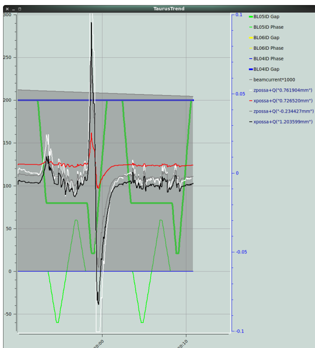
Figure 1: Effect of UARPES undulator movement without and with correction.
