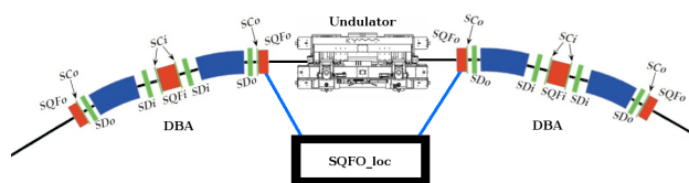
Figure 6: Connection of flanking SQFO magnets to power supply.
