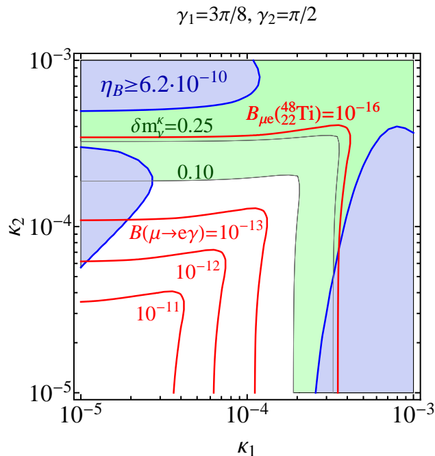
Figure 6. Contour plots of \kappa_1 versus \kappa_2 in a Minimal R \tau L model, with m_N = 120 GeV [13].
