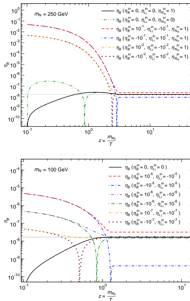
Figure 5. \eta_B versus z = m_{N_1}/T in the R\tau L model with m_N = 250 GeV (upper panel) and m_N = 100 GeV (lower panel).
