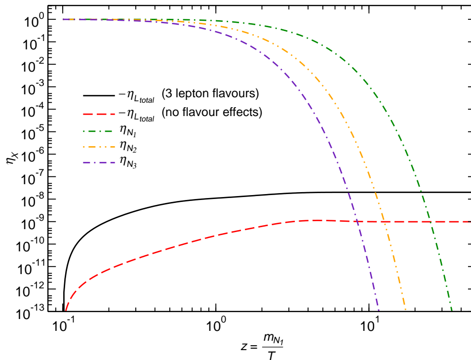
Figure 2. Numerical estimates for a scenario with m_{N_1} = 10^{10} GeV, m_{N_2} = 2m_{N_1} , m_{N_3} = 3m_{N_1} .
